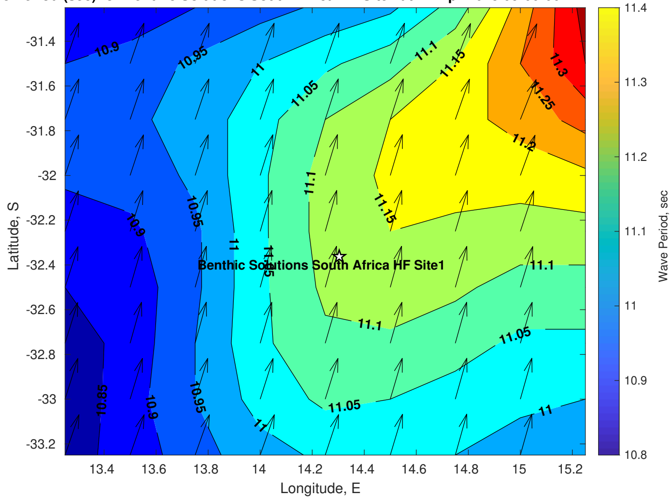
Wave Period (sec) for Benthic Solutions South Africa HF Site1 at 14-Apr-2025 09:00:00
