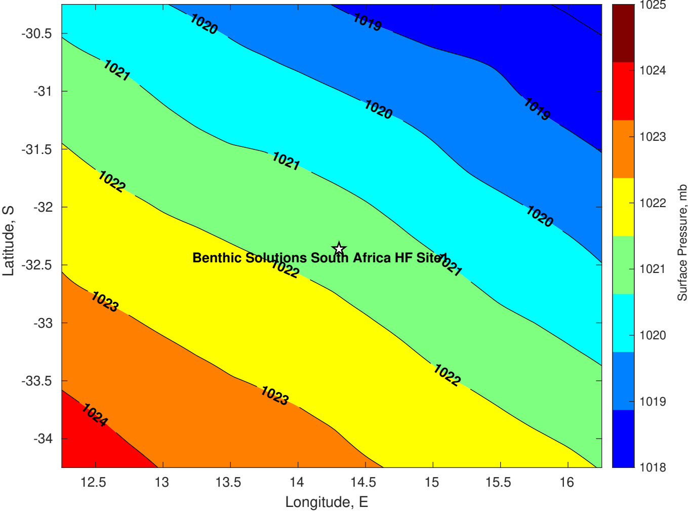
Surface Pressure (mb) for Benthic Solutions South Africa HF Site1 at 16-Apr-2025 00:00:00
