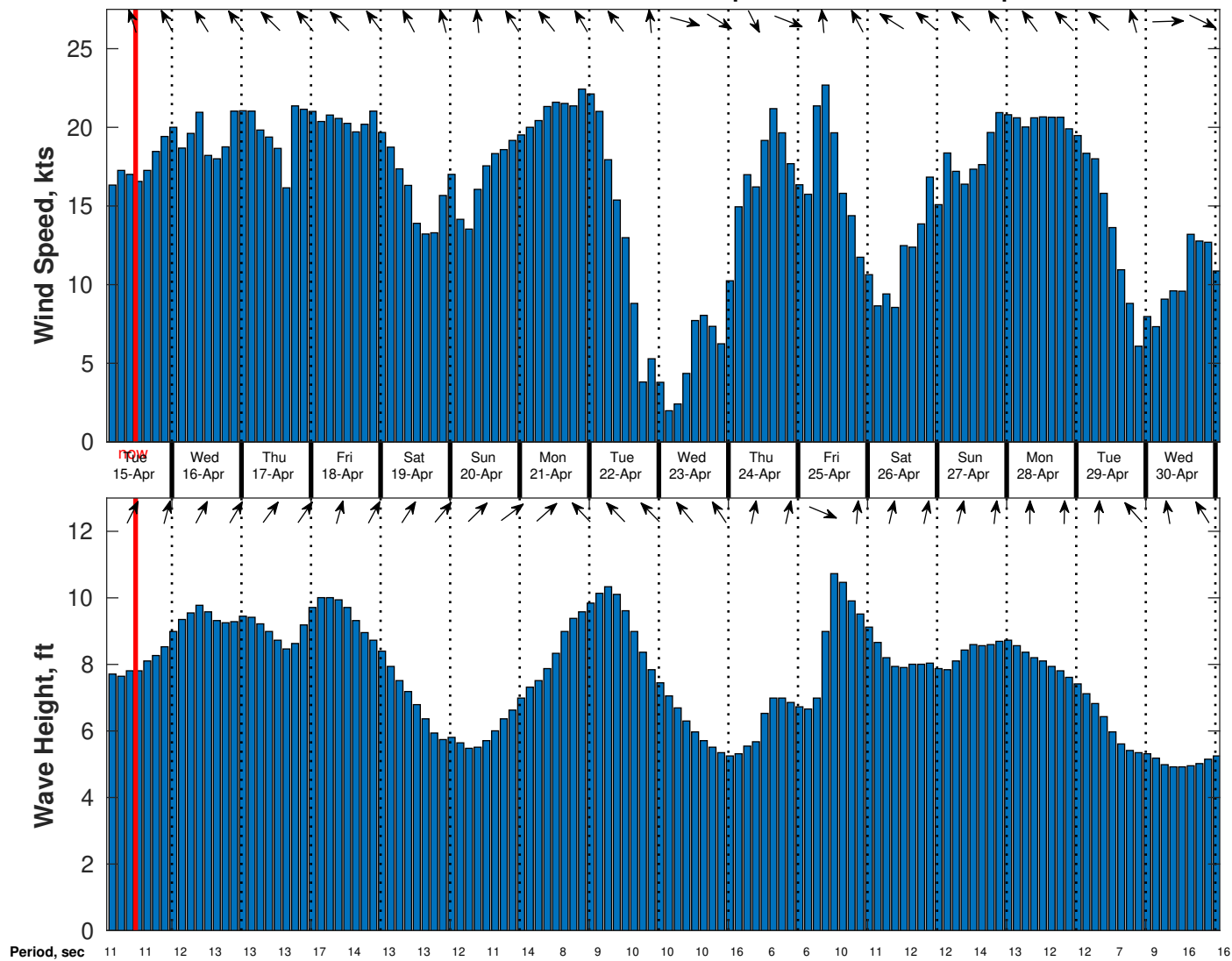
Wind & Wave Forecast for Benthic Solutions South Africa HF Site1 from 14-Apr-2025 02:00:00 to 30-Apr-2025 02:00:00
