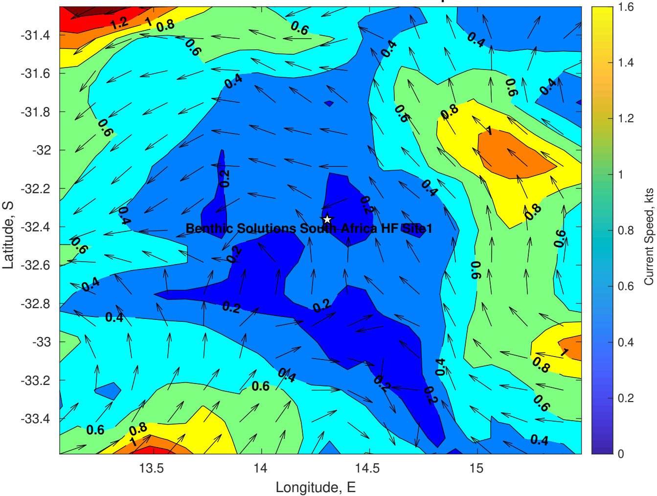
Surface Currents for Benthic Solutions South Africa HF Site1 at 13-Apr-2025 00:00:00
