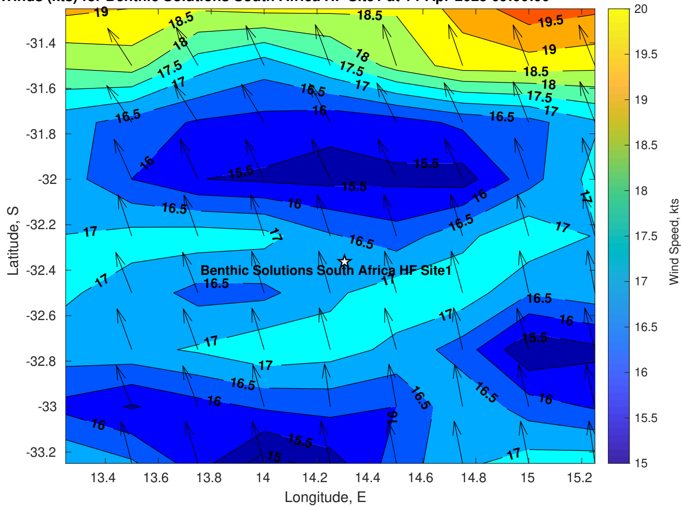
Winds (kts) for Benthic Solutions South Africa HF Site1 at 14-Apr-2025 09:00:00
