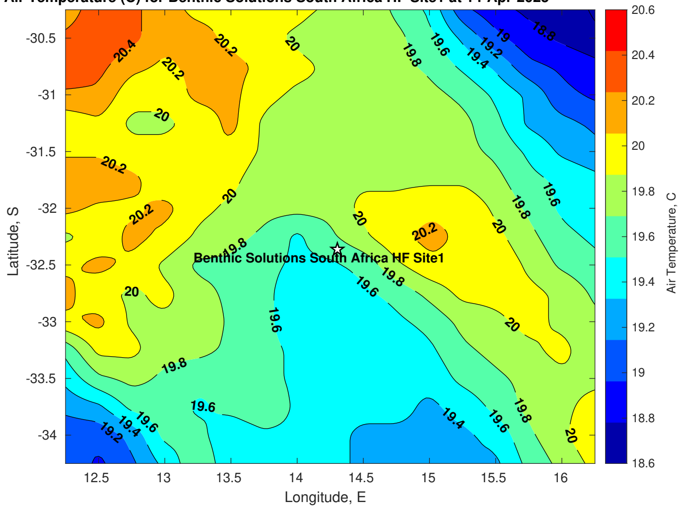
Air Temperature (C) for Benthic Solutions South Africa HF Site1 at 14-Apr-2025
