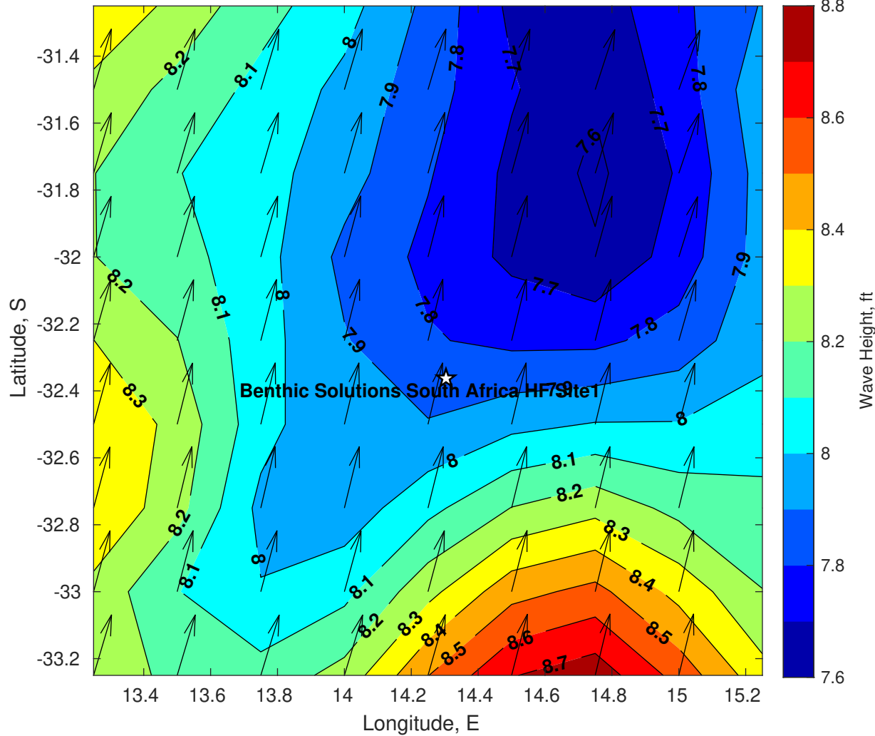
Wave Height (ft) for Benthic Solutions South Africa HF Site1 at 14-Apr-2025 09:00:00
