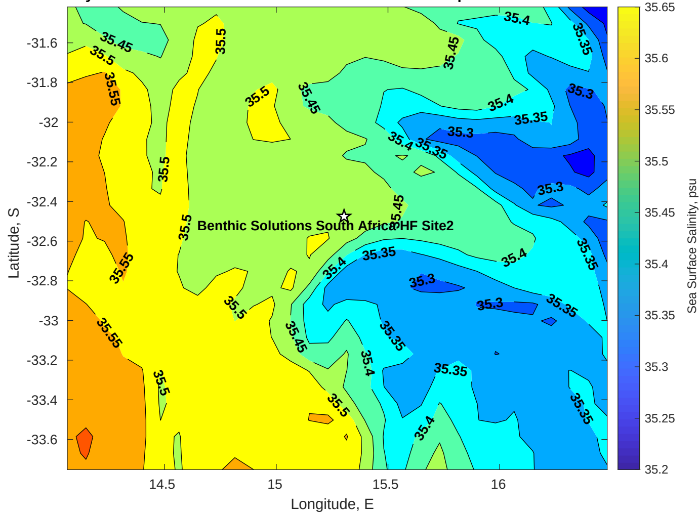
Surface Salinity for Benthic Solutions South Africa HF Site2 at 13-Apr-2025 00:00:00
