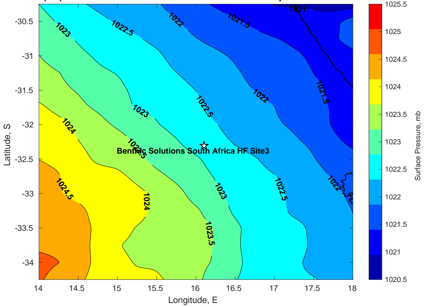
Surface Pressure (mb) for Benthic Solutions South Africa HF Site3 at 14-Apr-2025 00:00:00
