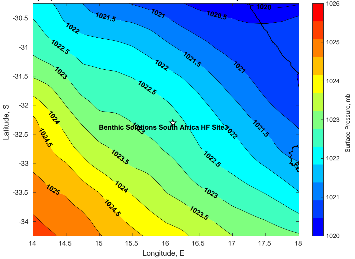
Surface Pressure (mb) for Benthic Solutions South Africa HF Site3 at 15-Apr-2025 00:00:00
