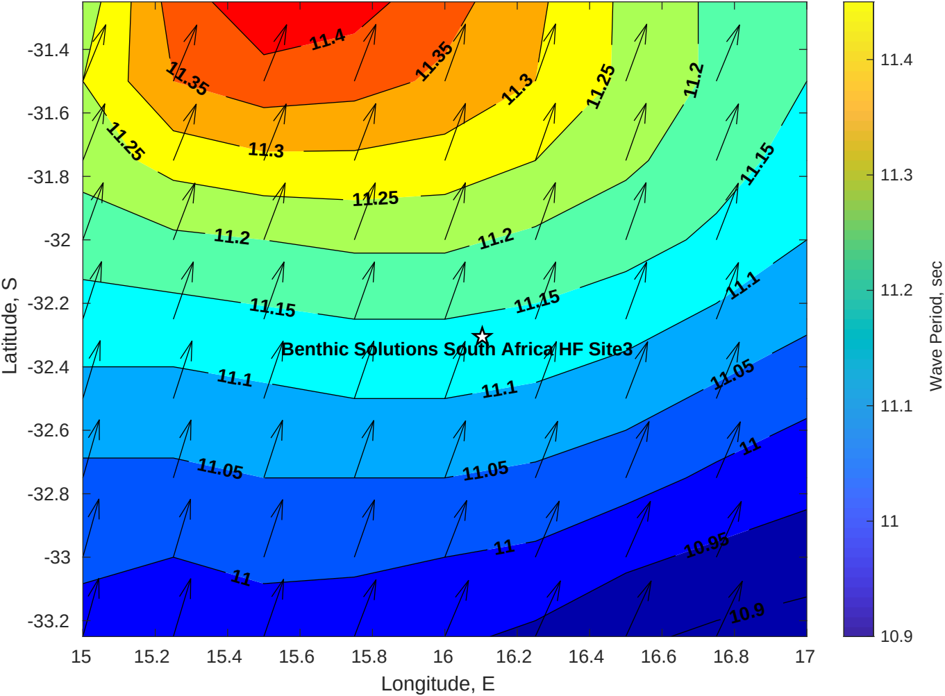
Wave Period (sec) for Benthic Solutions South Africa HF Site3 at 14-Apr-2025 09:00:00
