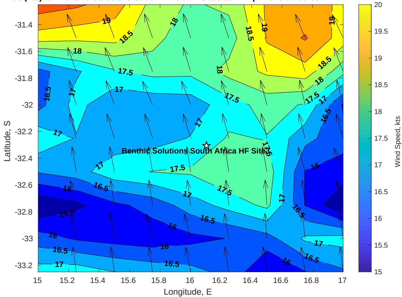
Winds (kts) for Benthic Solutions South Africa HF Site3 at 14-Apr-2025 09:00:00
