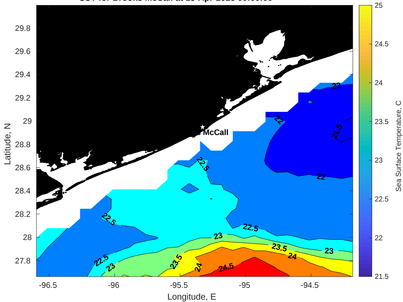
SST for Brooks McCall at 13-Apr-2025 00:00:00
