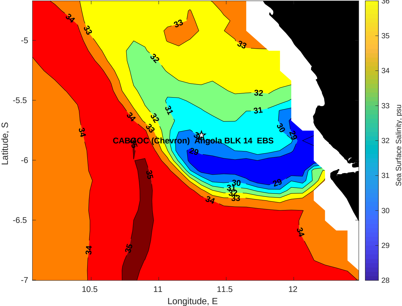
Surface Salinity for CABGOC (Chevron) Angola BLK 14 EBS at 13-Apr-2025 00:00:00
