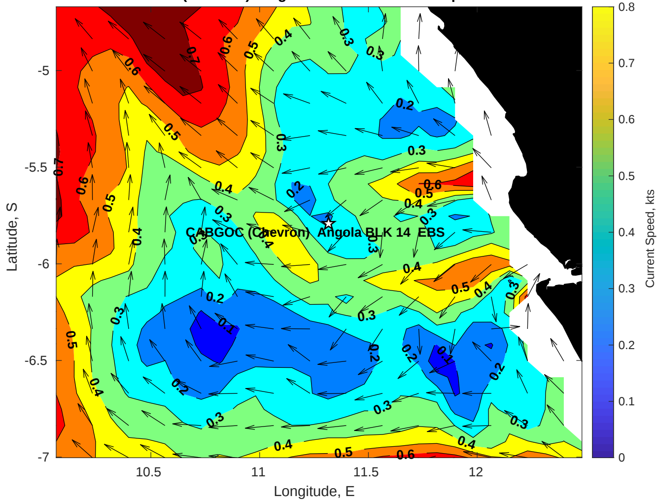
Surface Currents for CABGOC (Chevron) Angola BLK 14 EBS at 13-Apr-2025 00:00:00
