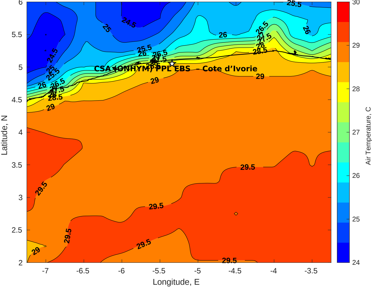
Air Temperature (C) for CSA (ONHYM) PPL EBS - Cote d'Ivoire at 14-Apr-2025
