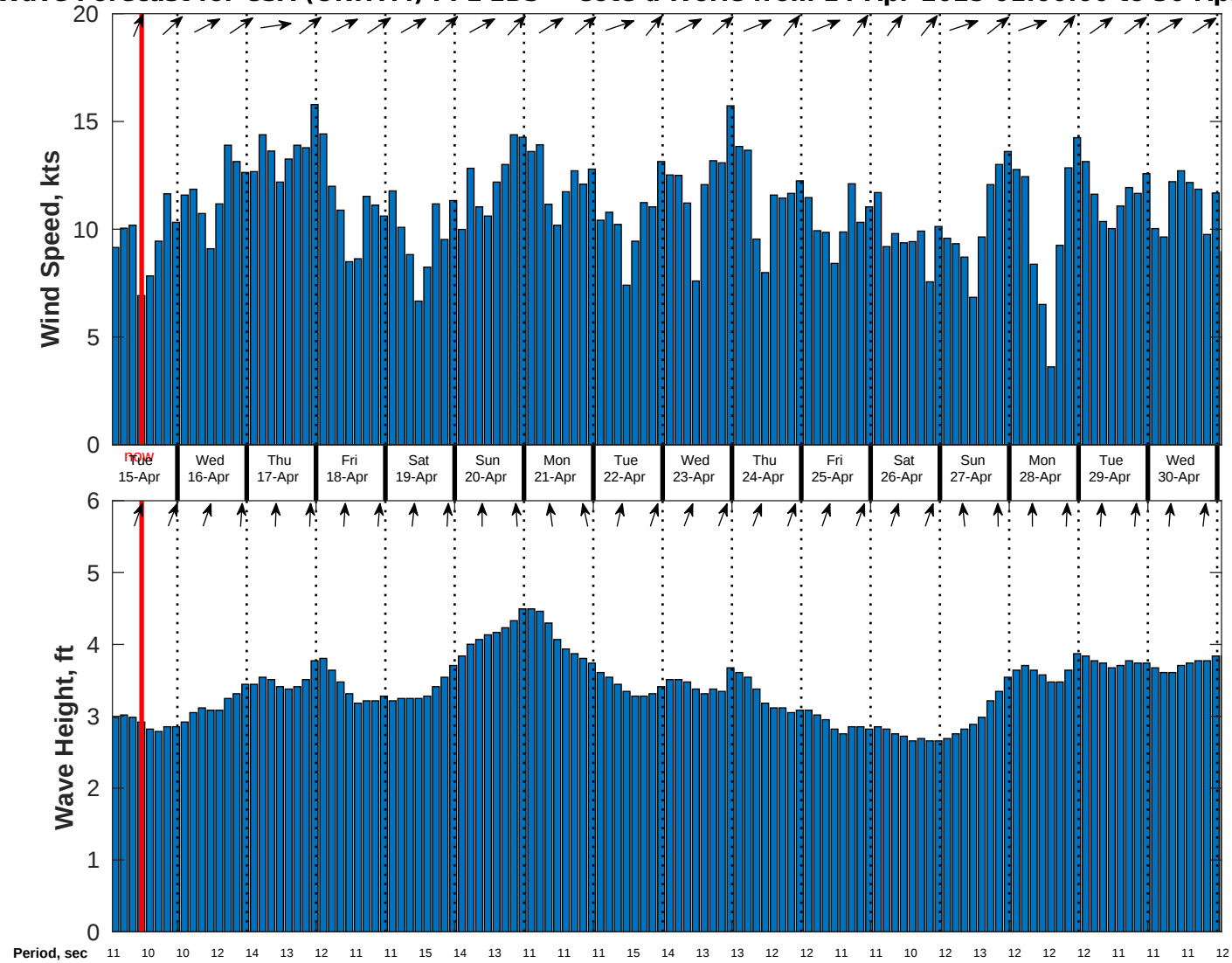
Wind & Wave Forecast for CSA (ONHYM) PPL EBS - Cote d'Ivoire from 14-Apr-2025 01:00:00 to 30-Apr-2025 01:00:00
