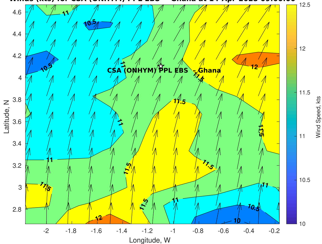
Winds (kts) for CSA (ONHYM) PPL EBS - Ghana at 14-Apr-2025 09:00:00
