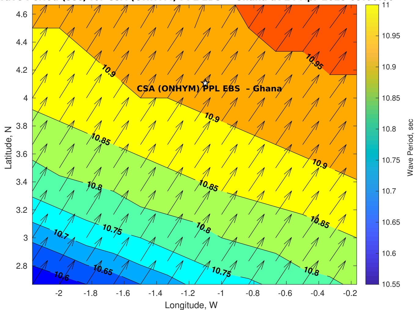
Wave Period (sec) for CSA (ONHYM) PPL EBS - Ghana at 14-Apr-2025 09:00:00
