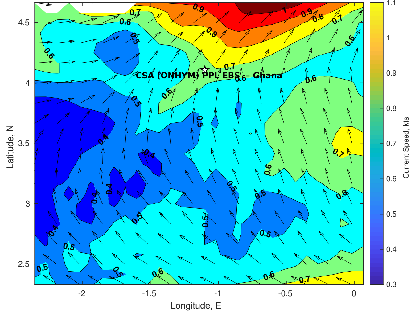
Surface Currents for CSA (ONHYM) PPL EBS - Ghana at 13-Apr-2025 00:00:00
