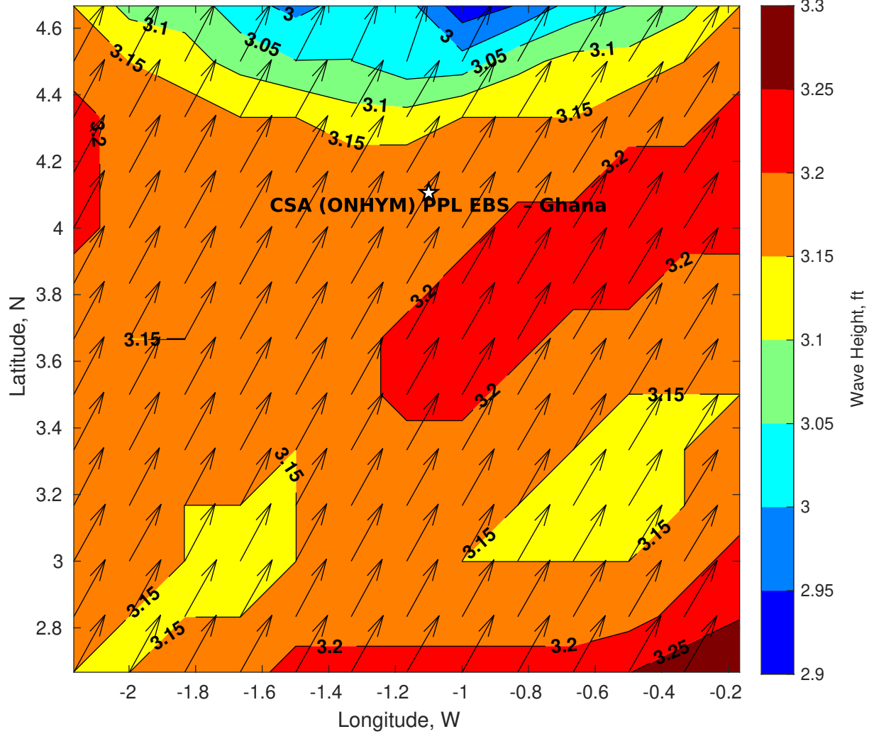
Wave Height (ft) for CSA (ONHYM) PPL EBS - Ghana at 14-Apr-2025 09:00:00
