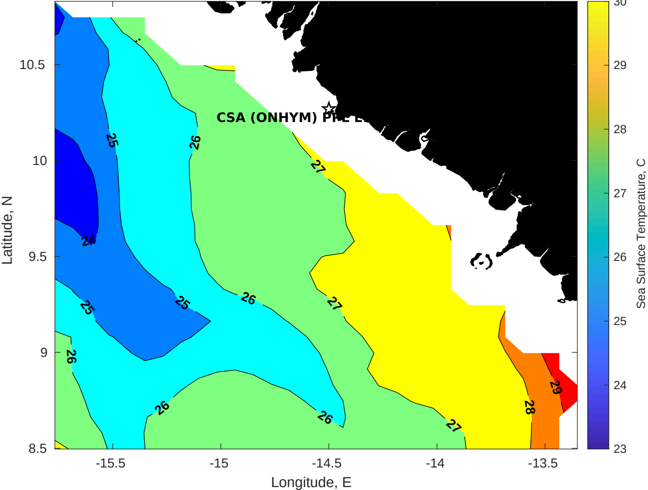
SST for CSA (ONHYM) PPL EBS - Guinea at 13-Apr-2025 00:00:00
