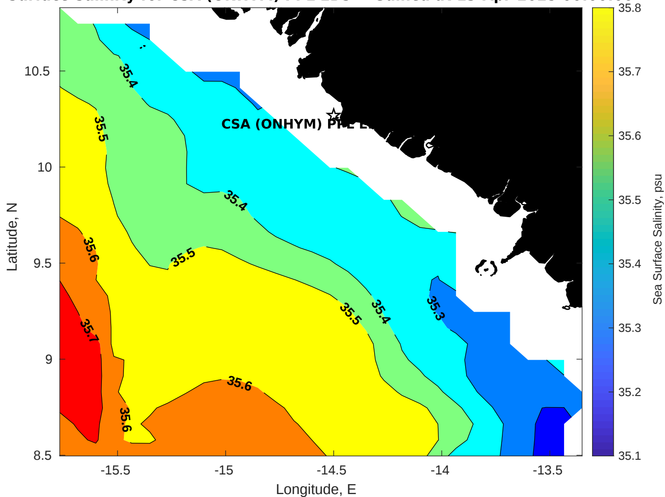
Surface Salinity for CSA (ONHYM) PPL EBS - Guinea at 13-Apr-2025 00:00:00
