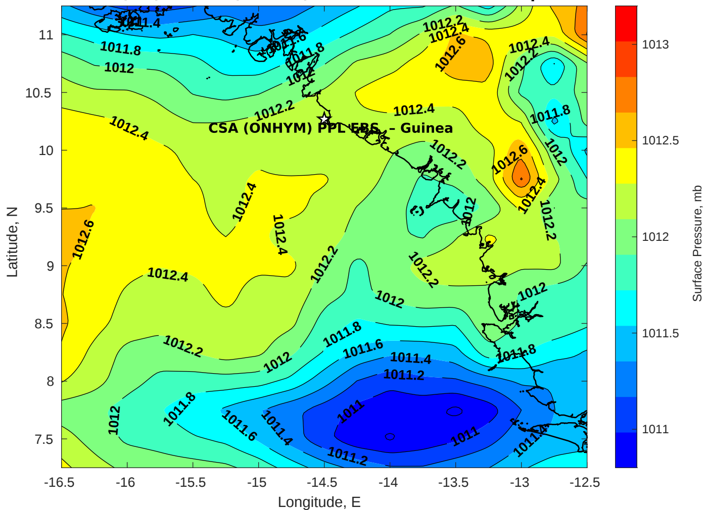
Surface Pressure (mb) for CSA (ONHYM) PPL EBS - Guinea at 14-Apr-2025 00:00:00
