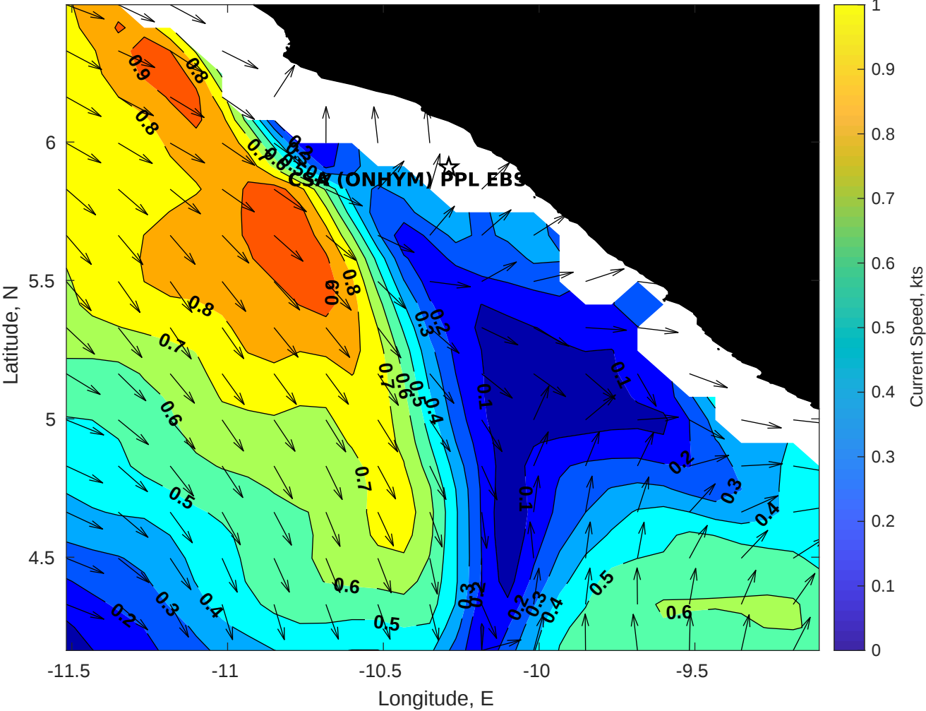
Surface Currents for CSA (ONHYM) PPL EBS - Liberia at 13-Apr-2025 00:00:00
