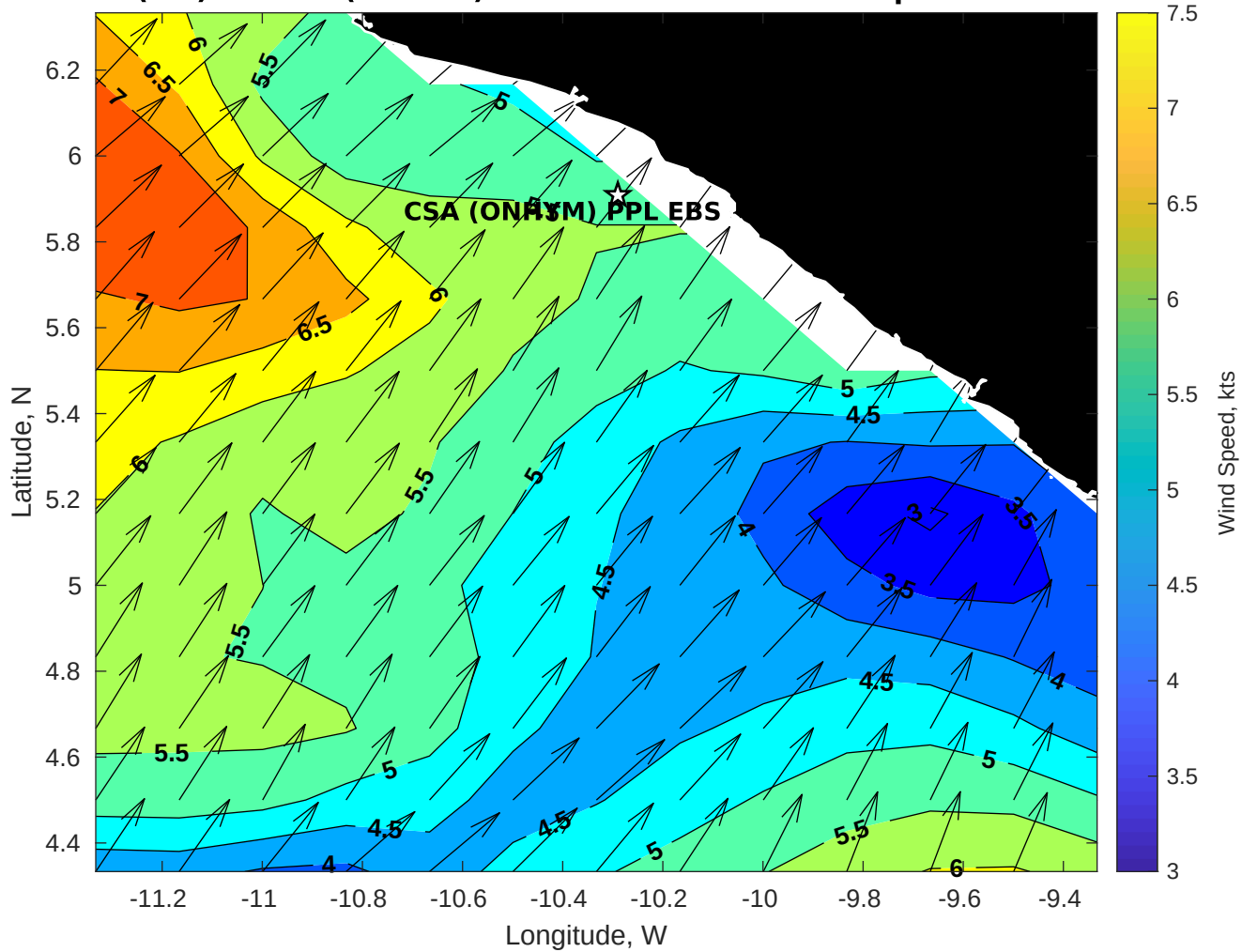
Winds (kts) for CSA (ONHYM) PPL EBS - Liberia at 14-Apr-2025 09:00:00
