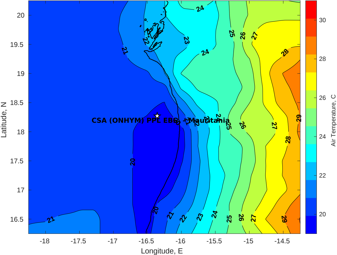
Air Temperature (C) for CSA (ONHYM) PPL EBS - Mauritania at 14-Apr-2025
