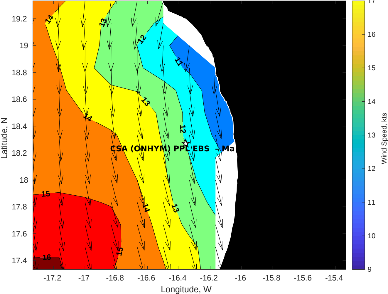
Winds (kts) for CSA (ONHYM) PPL EBS - Mauritania at 14-Apr-2025 09:00:00
