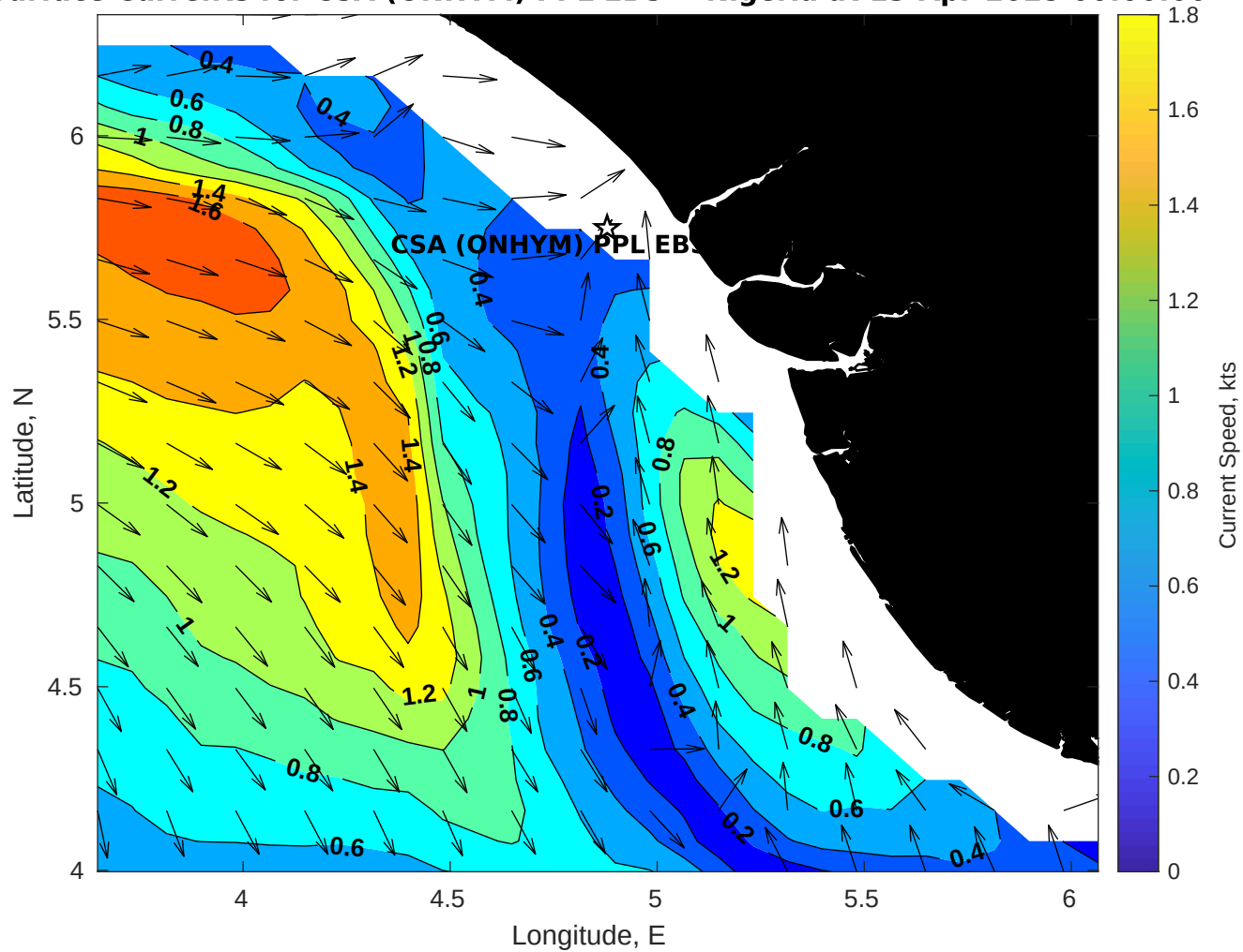
Surface Currents for CSA (ONHYM) PPL EBS - Nigeria at 13-Apr-2025 00:00:00
