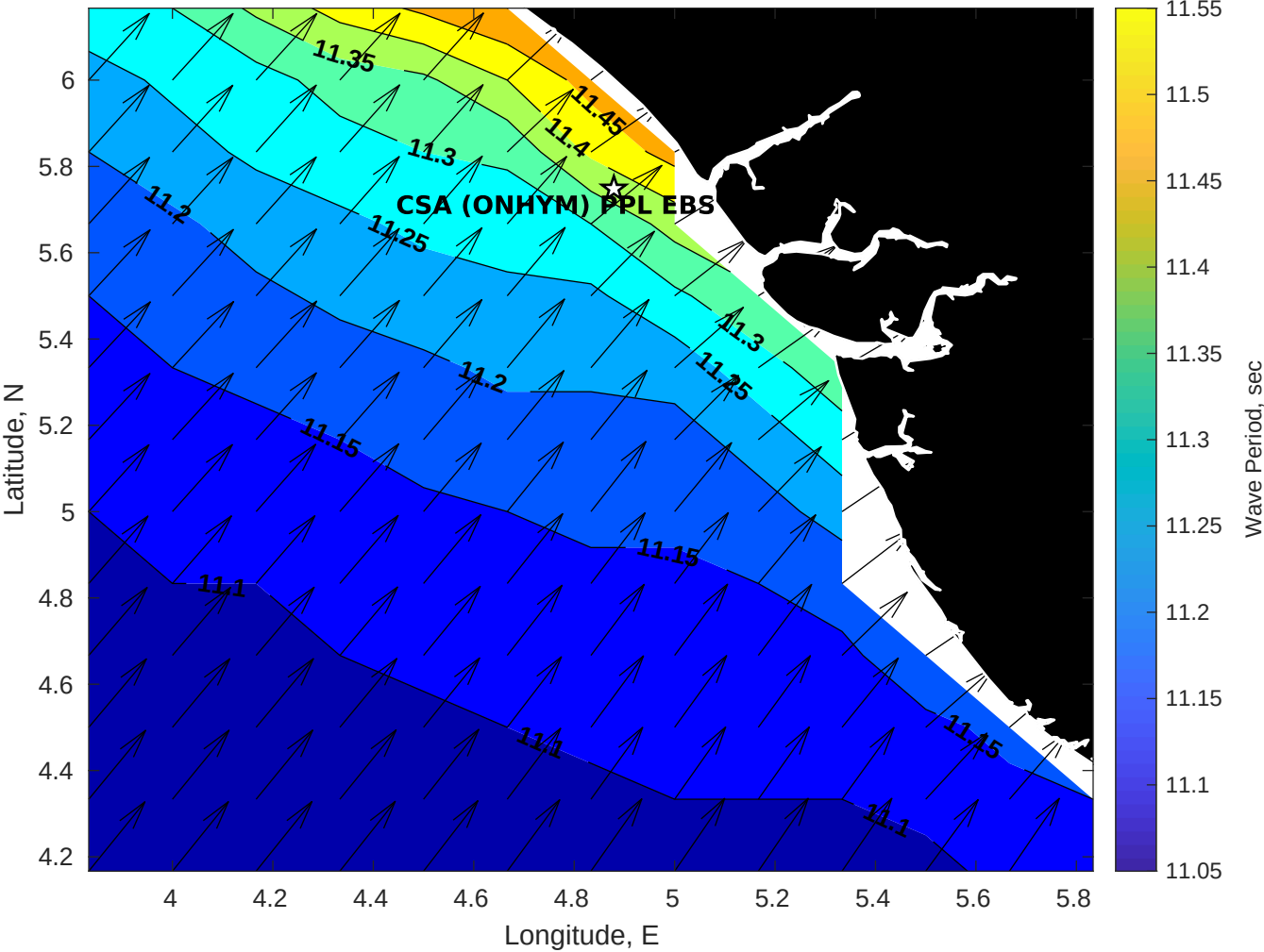
Wave Period (sec) for CSA (ONHYM) PPL EBS - Nigeria at 14-Apr-2025 09:00:00
