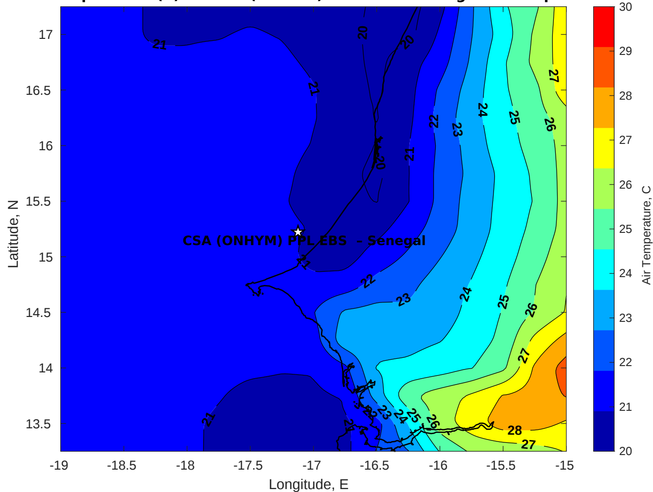
Air Temperature (C) for CSA (ONHYM) PPL EBS - Senegal at 14-Apr-2025
