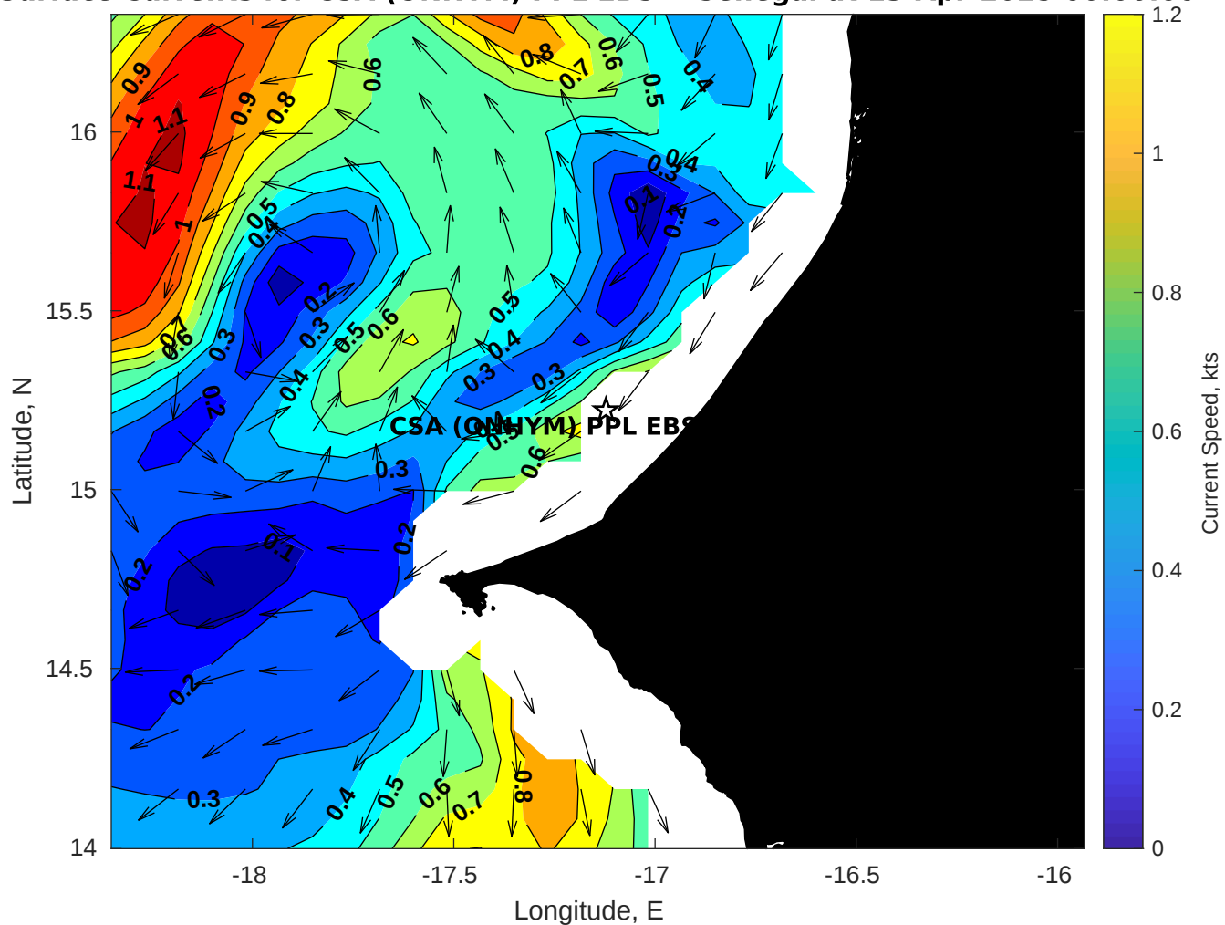
Surface Currents for CSA (ONHYM) PPL EBS - Senegal at 13-Apr-2025 00:00:00
