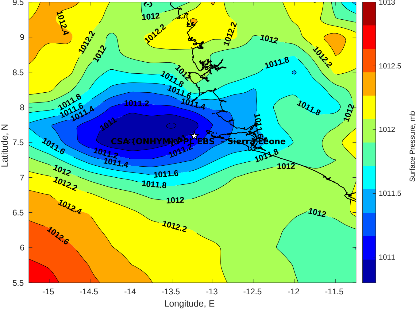
Surface Pressure (mb) for CSA (ONHYM) PPL EBS - Sierra Leone at 14-Apr-2025 00:00:00
