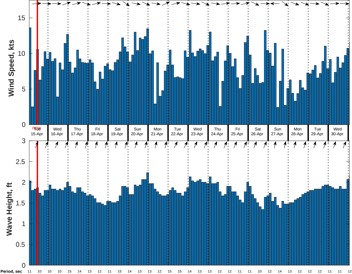
Wind & Wave Forecast for CSA (ONHYM) PPL EBS - Sierra Leone from 14-Apr-2025 01:00:00 to 30-Apr-2025 01:00:00
