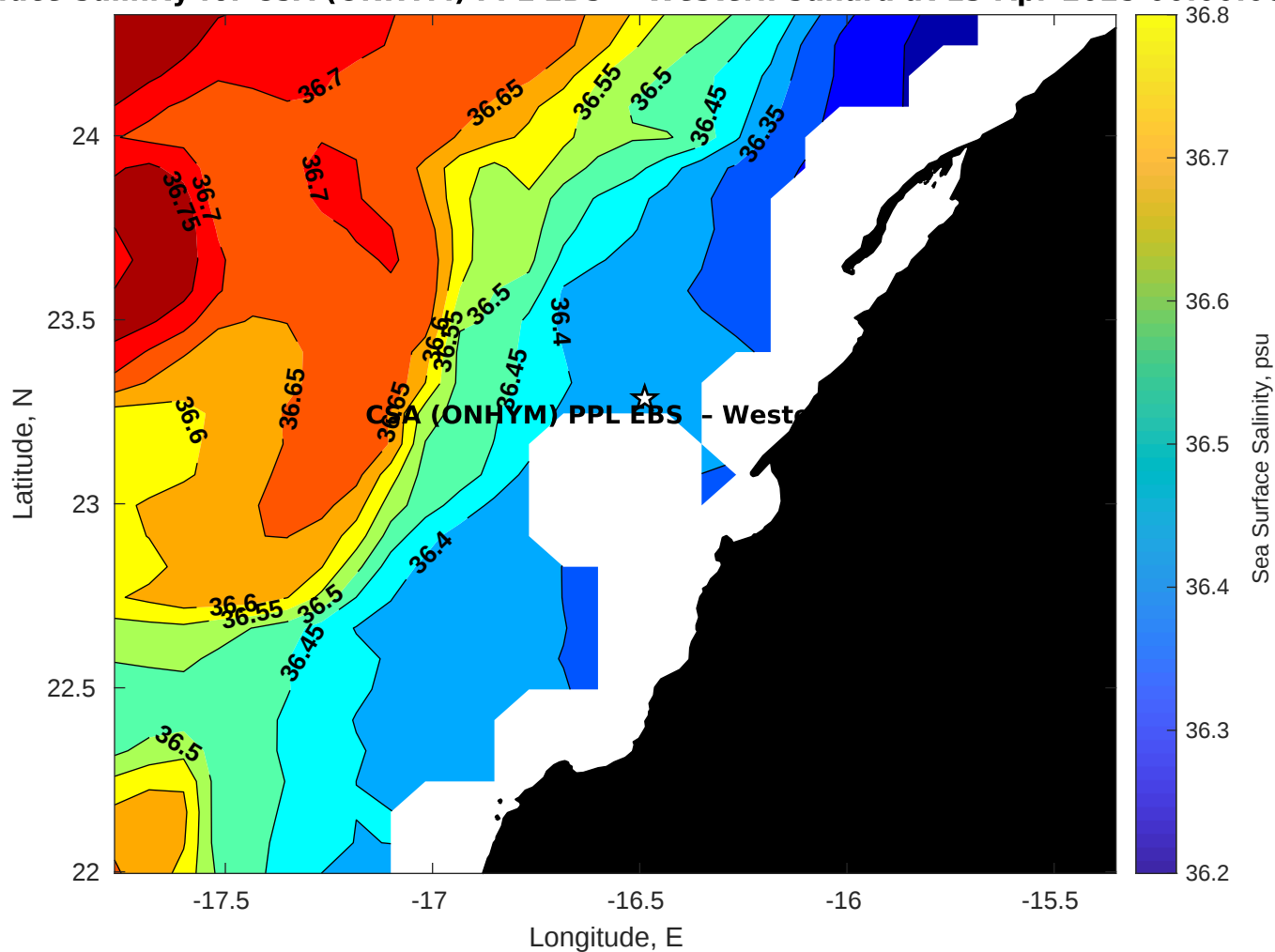
Surface Salinity for CSA (ONHYM) PPL EBS - Western Sahara at 13-Apr-2025 00:00:00
