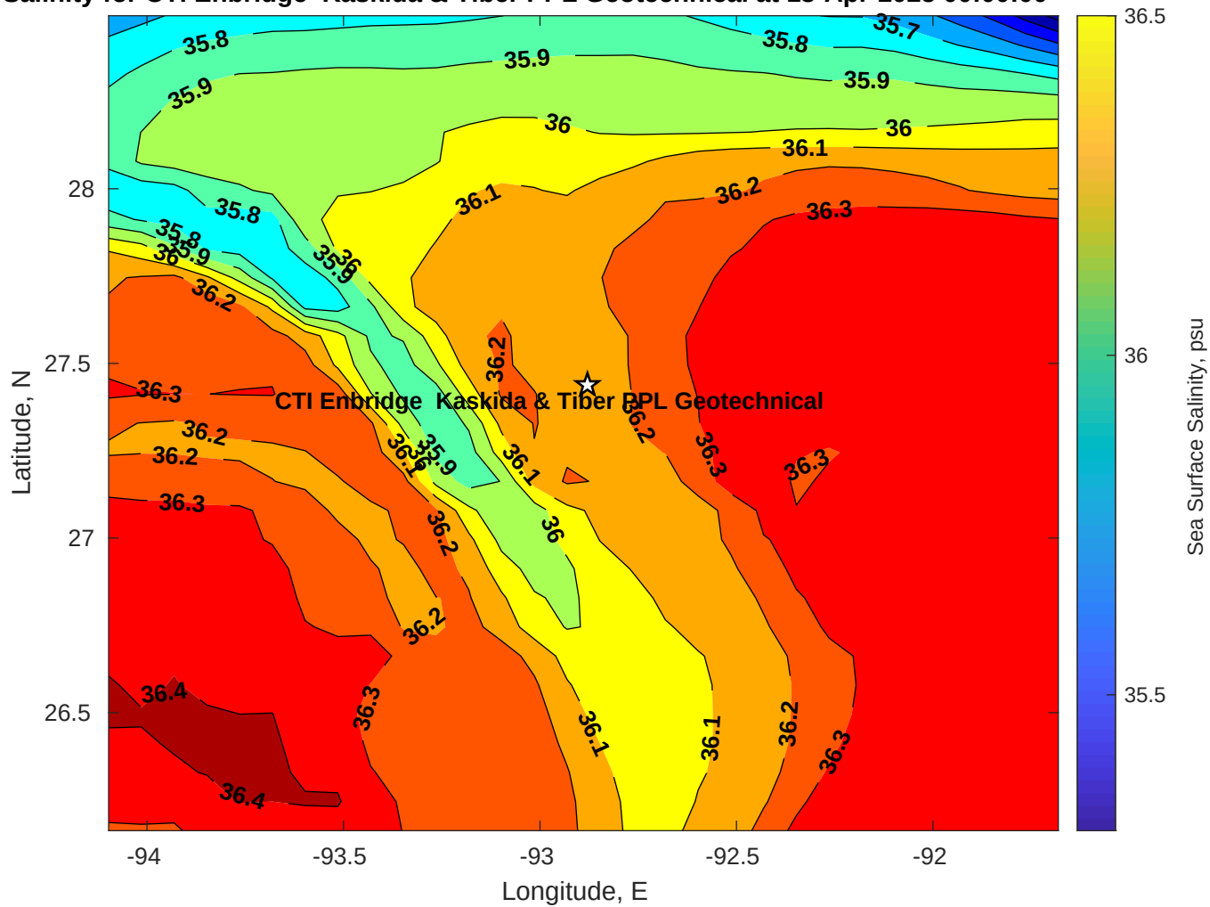
Surface Salinity for CTI Enbridge Kaskida & Tiber PPL Geotechnical at 13-Apr-2025 00:00:00
