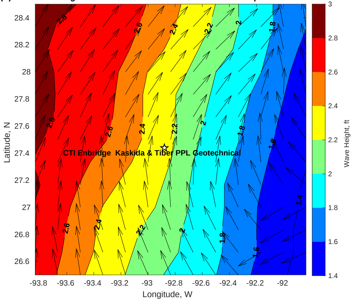
Wave Height (ft) for CTI Enbridge Kaskida & Tiber PPL Geotechnical at 14-Apr-2025 09:00:00
