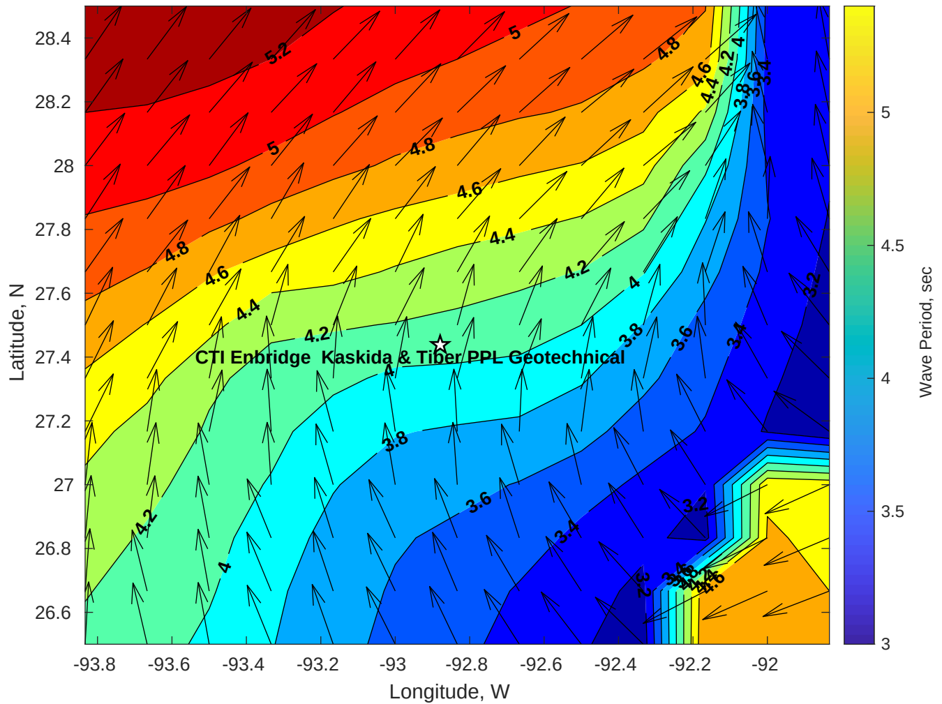
Wave Period (sec) for CTI Enbridge Kaskida & Tiber PPL Geotechnical at 14-Apr-2025 09:00:00
