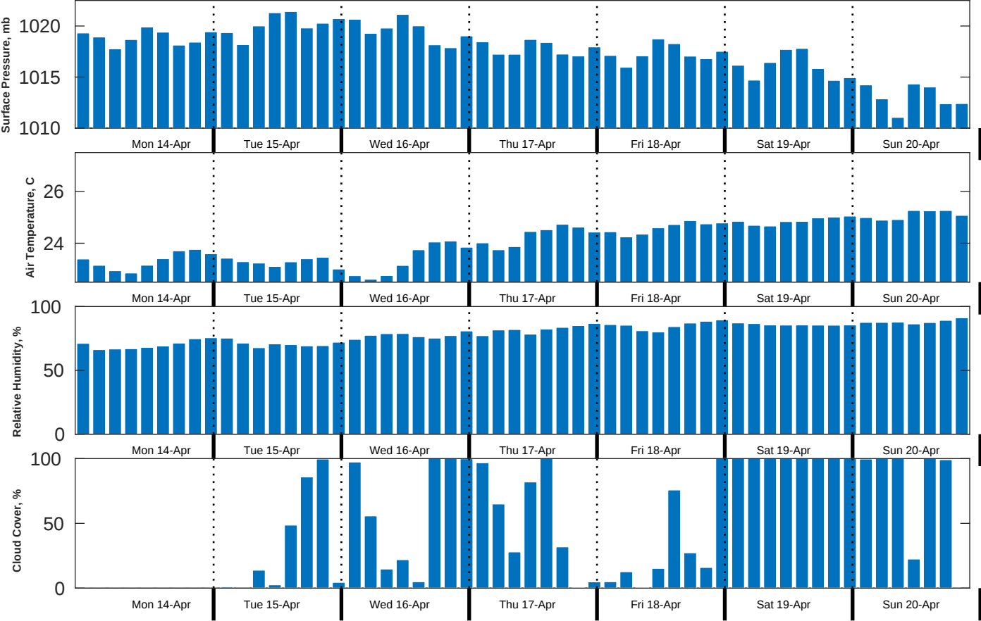
Met Forecast for CTI Enbridge Kaskida & Tiber PPL Geotechnical from 14-Apr-2025 00:00:00 to 21-Apr-2025 00:00:00
