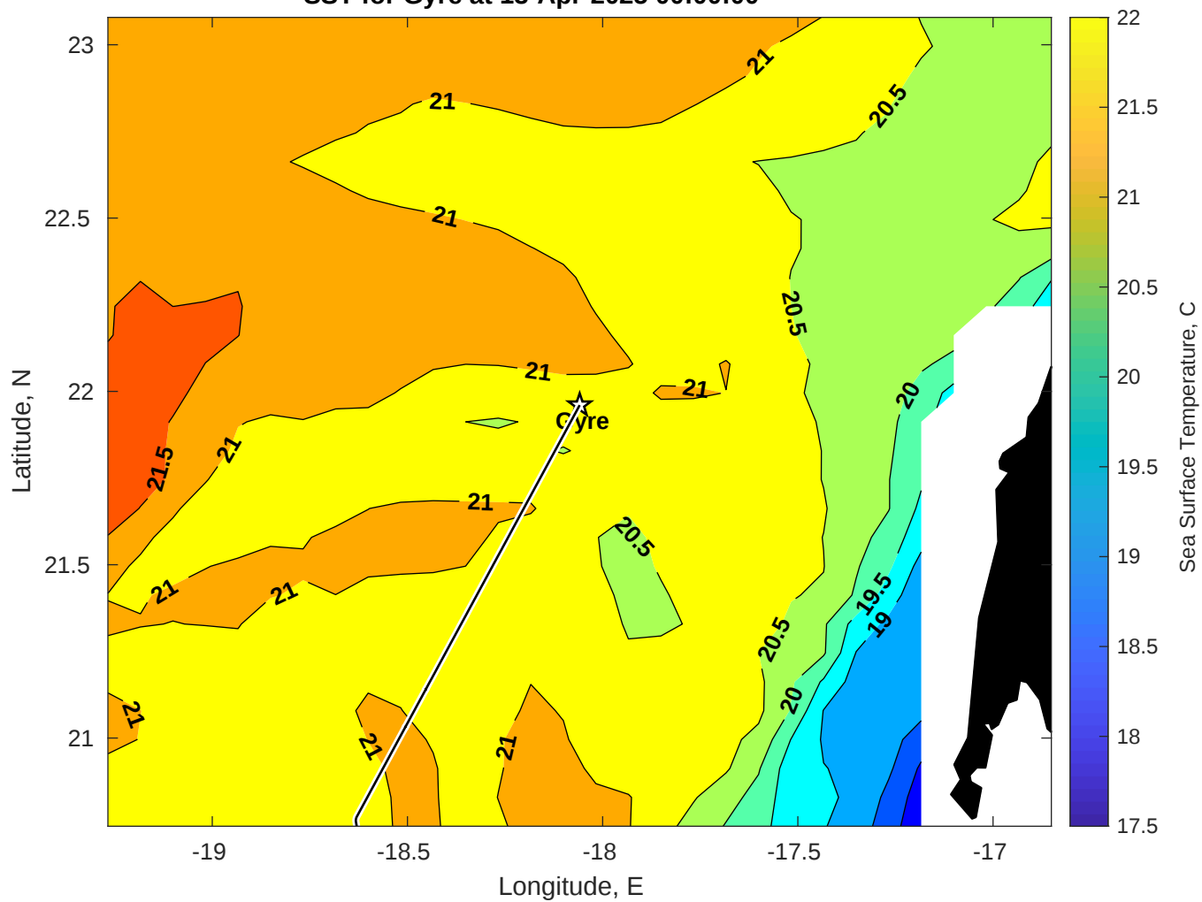
SST for Gyre at 13-Apr-2025 00:00:00
