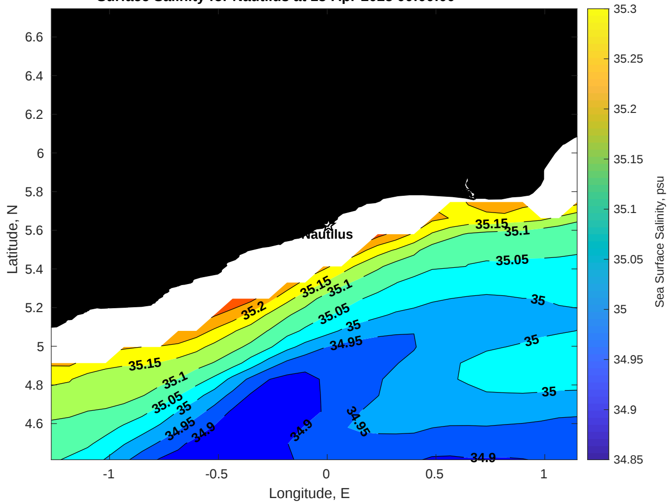
Surface Salinity for Nautilus at 13-Apr-2025 00:00:00
