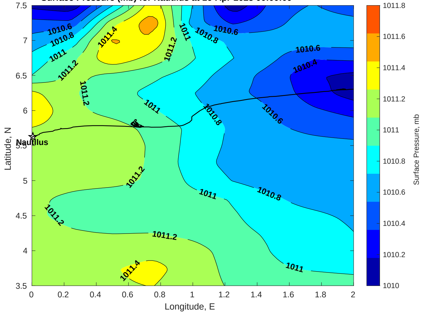
Surface Pressure (mb) for Nautilus at 16-Apr-2025 00:00:00
