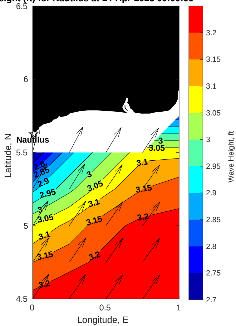
Wave Height (ft) for Nautilus at 14-Apr-2025 09:00:00
