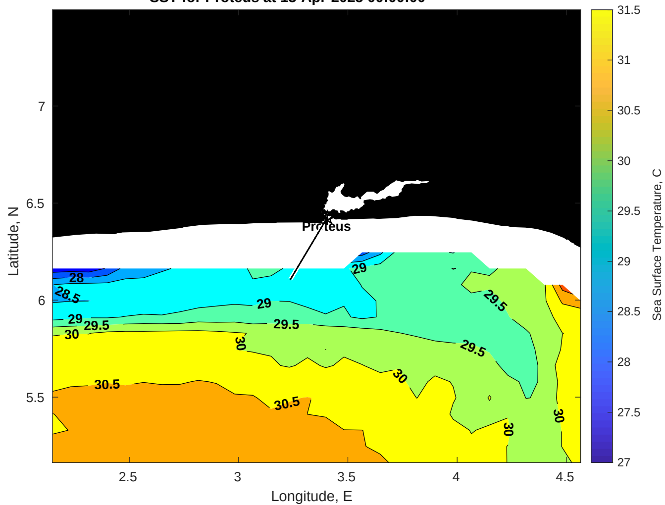
SST for Proteus at 13-Apr-2025 00:00:00
