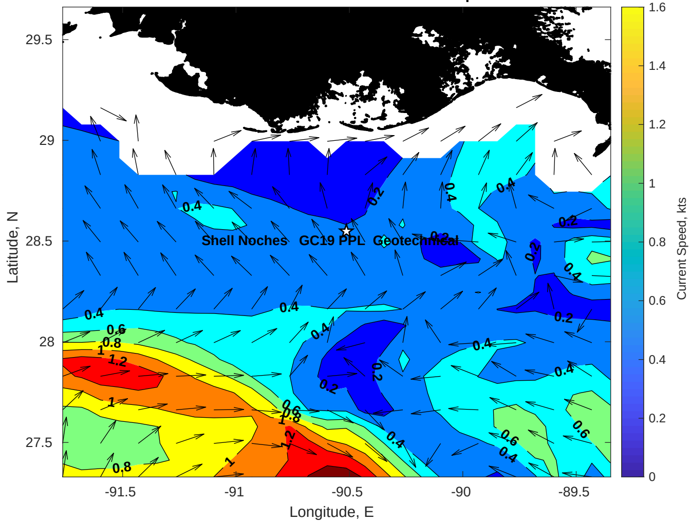
Surface Currents for Shell Noches GC19 PPL Geotechnical at 13-Apr-2025 00:00:00
