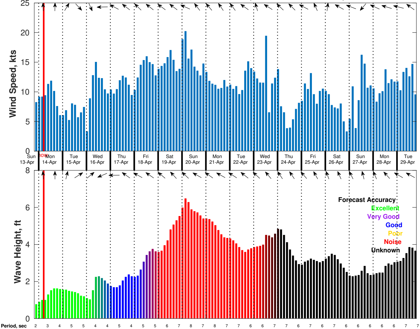
Wind & Wave Forecast for Shell Noches GC19 PPL Geotechnical from 13-Apr-2025 20:00:00 to 29-Apr-2025 20:00:00
