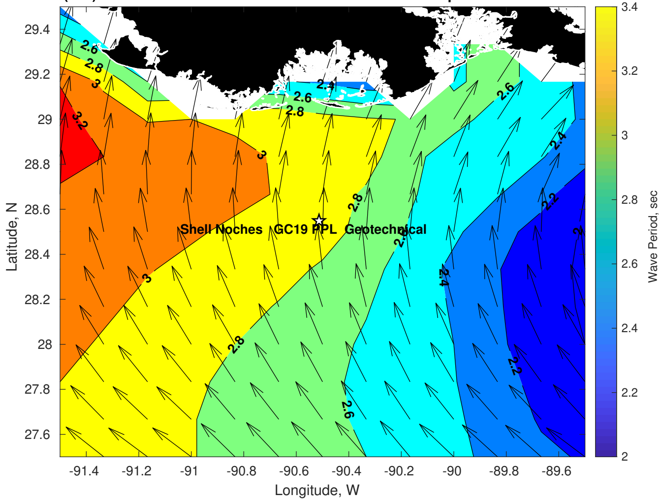
Wave Period (sec) for Shell Noches GC19 PPL Geotechnical at 14-Apr-2025 09:00:00
