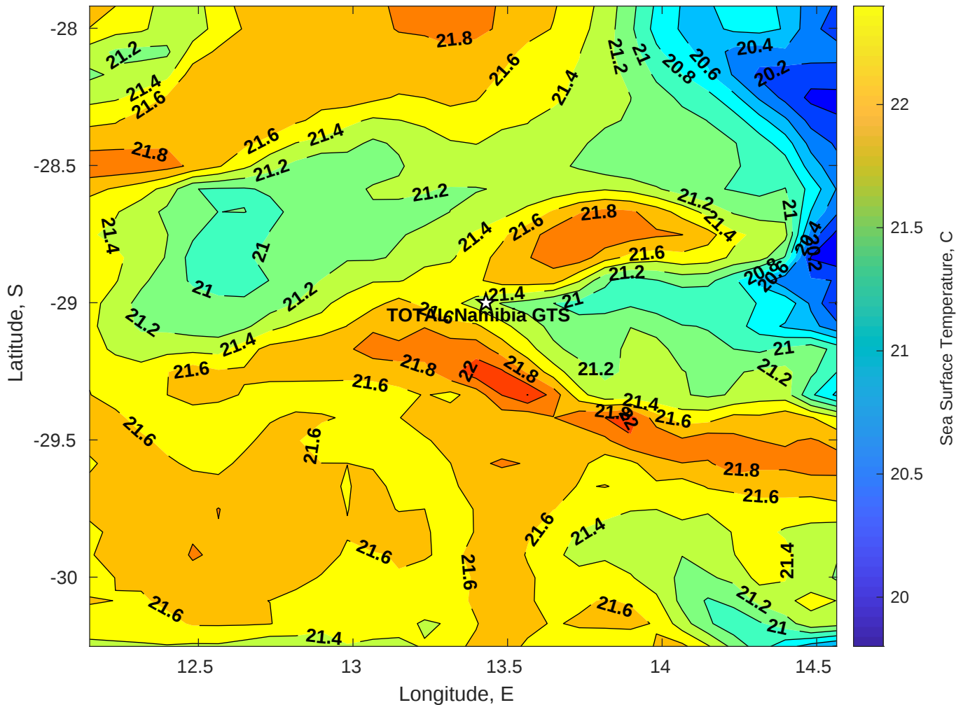
SST for TOTAL Namibia GTS at 13-Apr-2025 00:00:00
