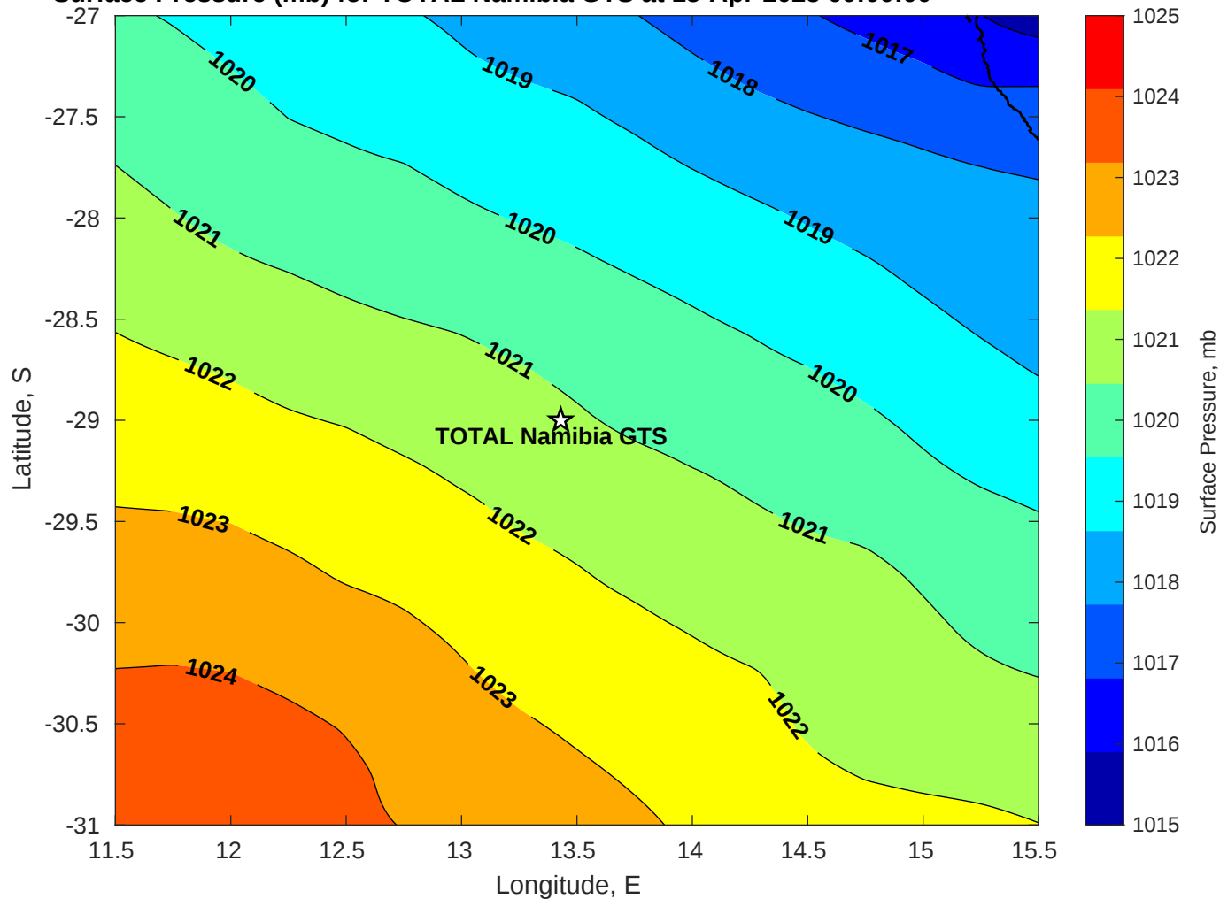
Surface Pressure (mb) for TOTAL Namibia GTS at 15-Apr-2025 00:00:00
