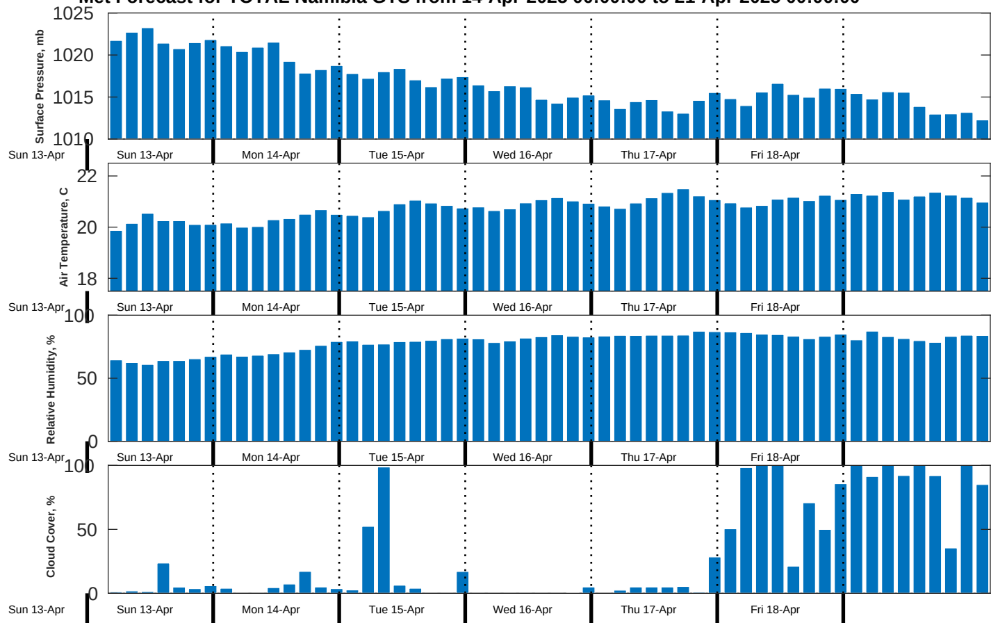
Met Forecast for TOTAL Namibia GTS from 14-Apr-2025 00:00:00 to 21-Apr-2025 00:00:00
