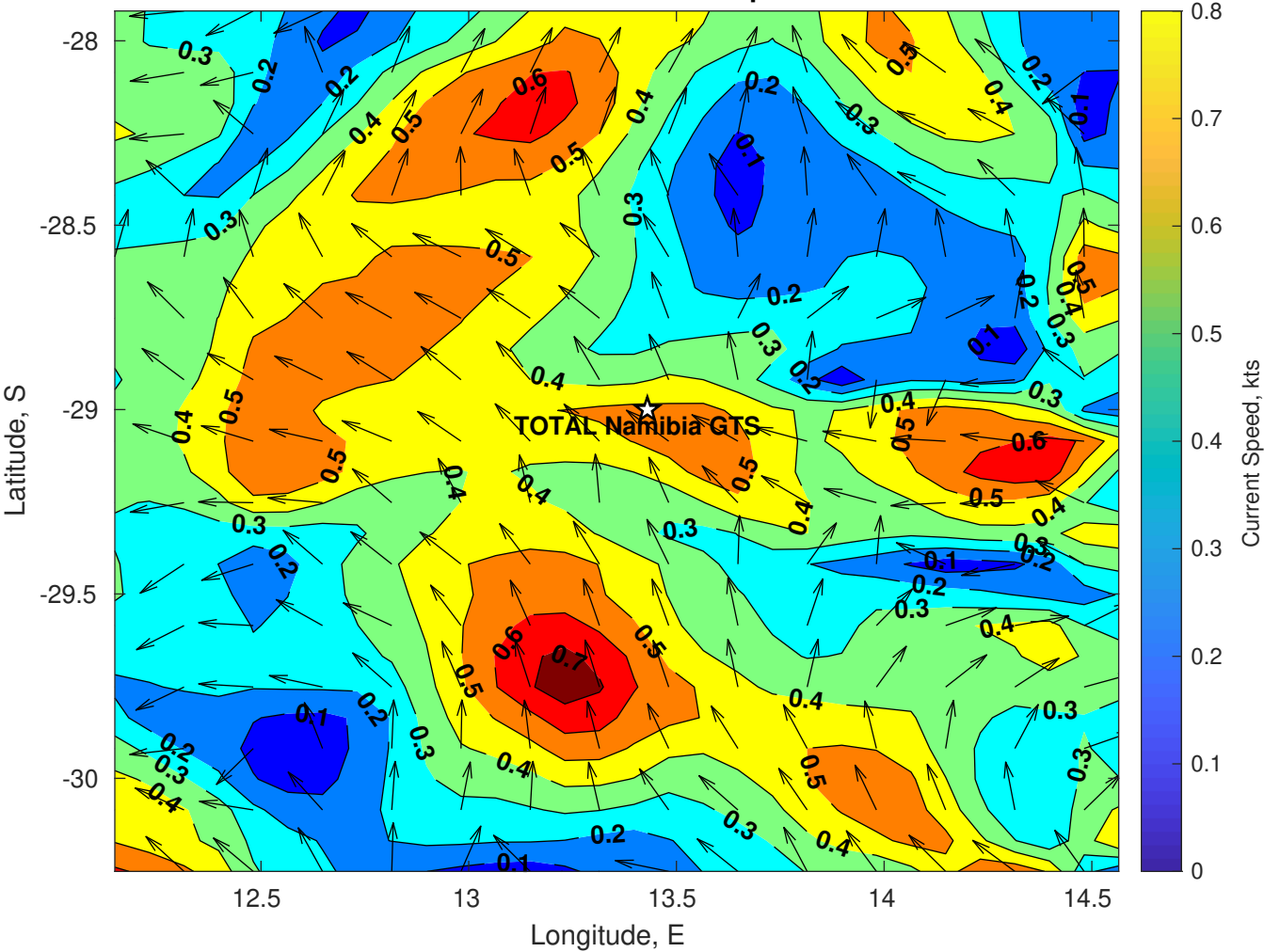
Surface Currents for TOTAL Namibia GTS at 13-Apr-2025 00:00:00
