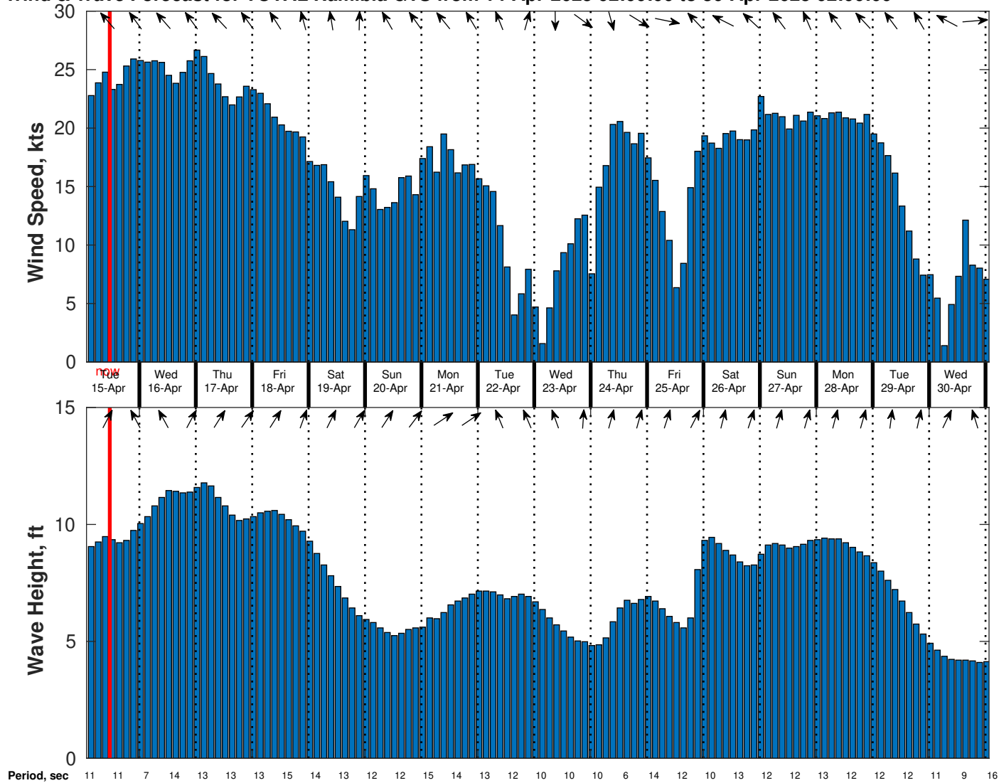
Wind & Wave Forecast for TOTAL Namibia GTS from 14-Apr-2025 02:00:00 to 30-Apr-2025 02:00:00
