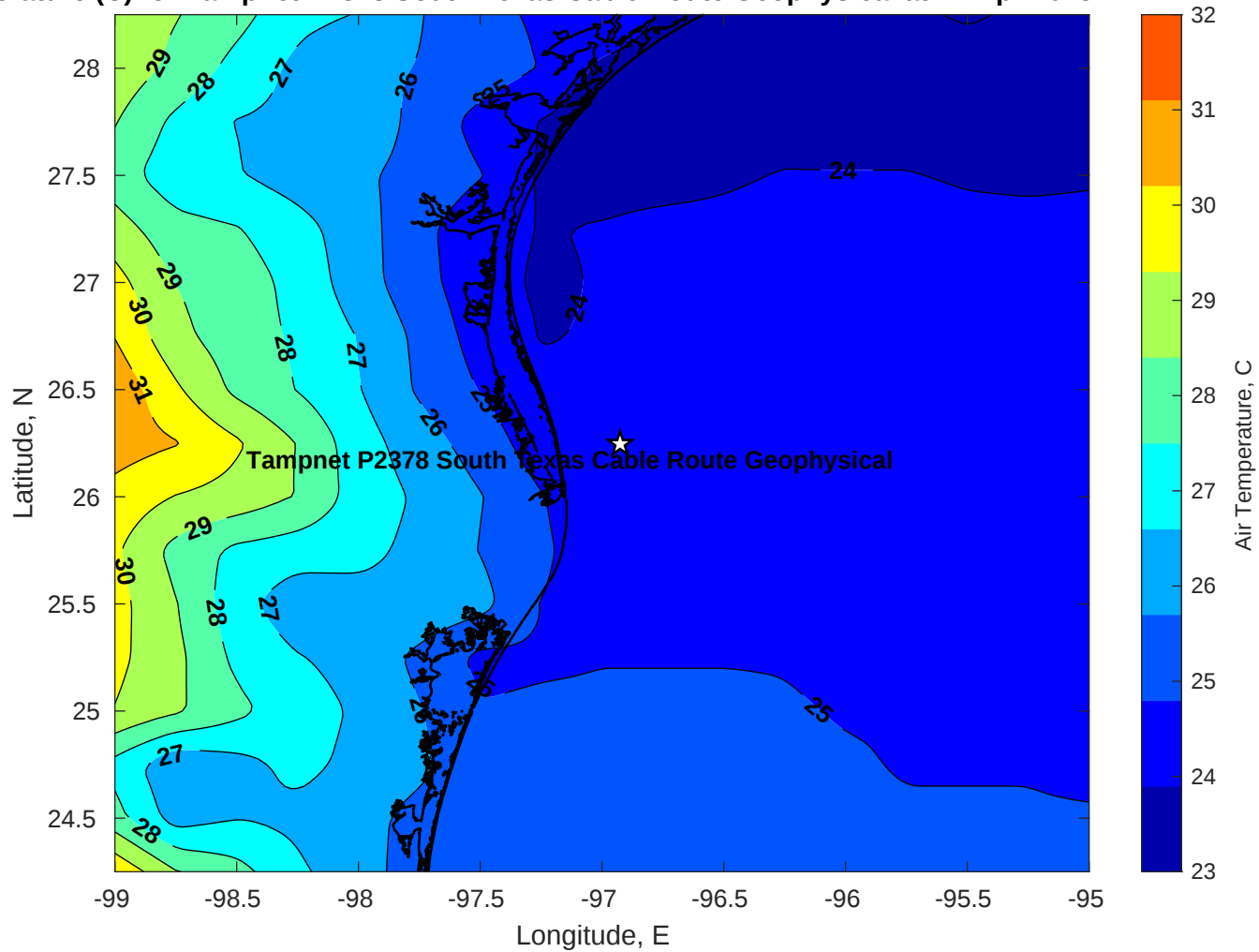
Air Temperature (C) for Tampnet P2378 South Texas Cable Route Geophysical at 14-Apr-2025
