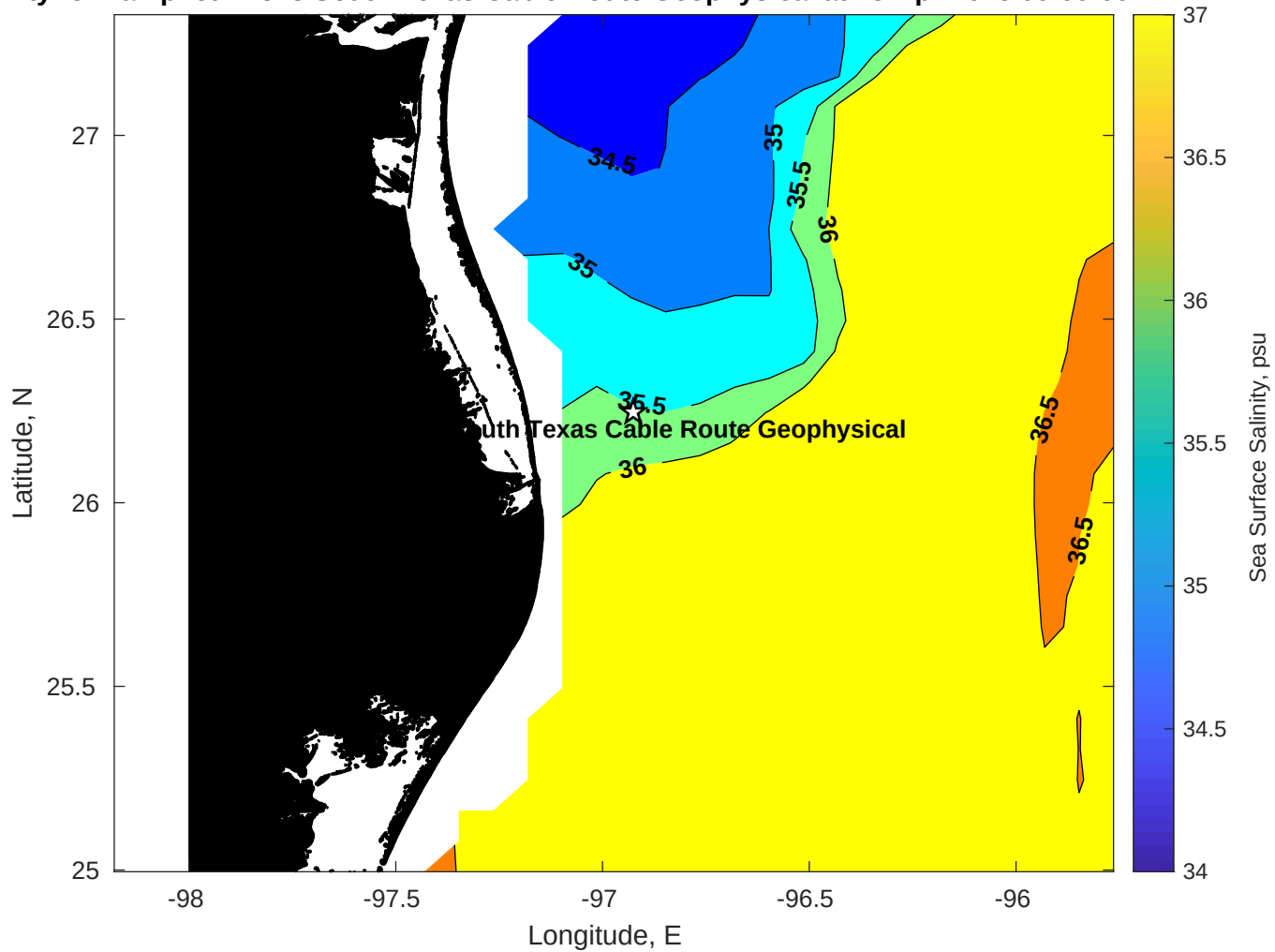
Surface Salinity for Tampnet P2378 South Texas Cable Route Geophysical at 13-Apr-2025 00:00:00
