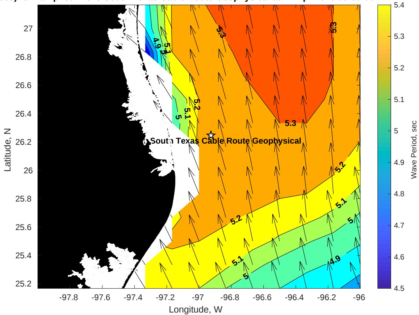
Period (sec) for Tampnet P2378 South Texas Cable Route Geophysical at 14-Apr-2025 09:00:00
