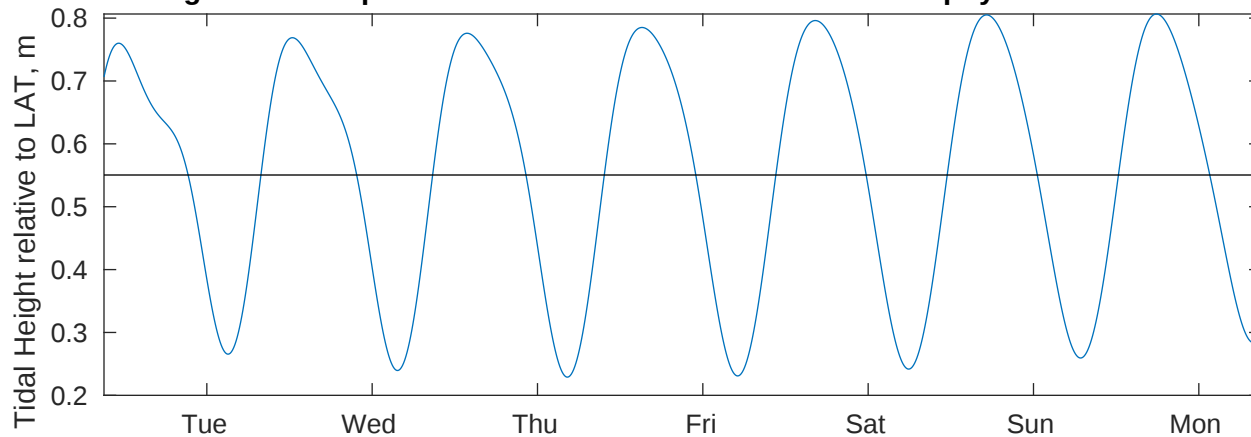
Tidal Currents and Heights for Tampnet P2378 South Texas Cable Route Geophysical at 20250414
