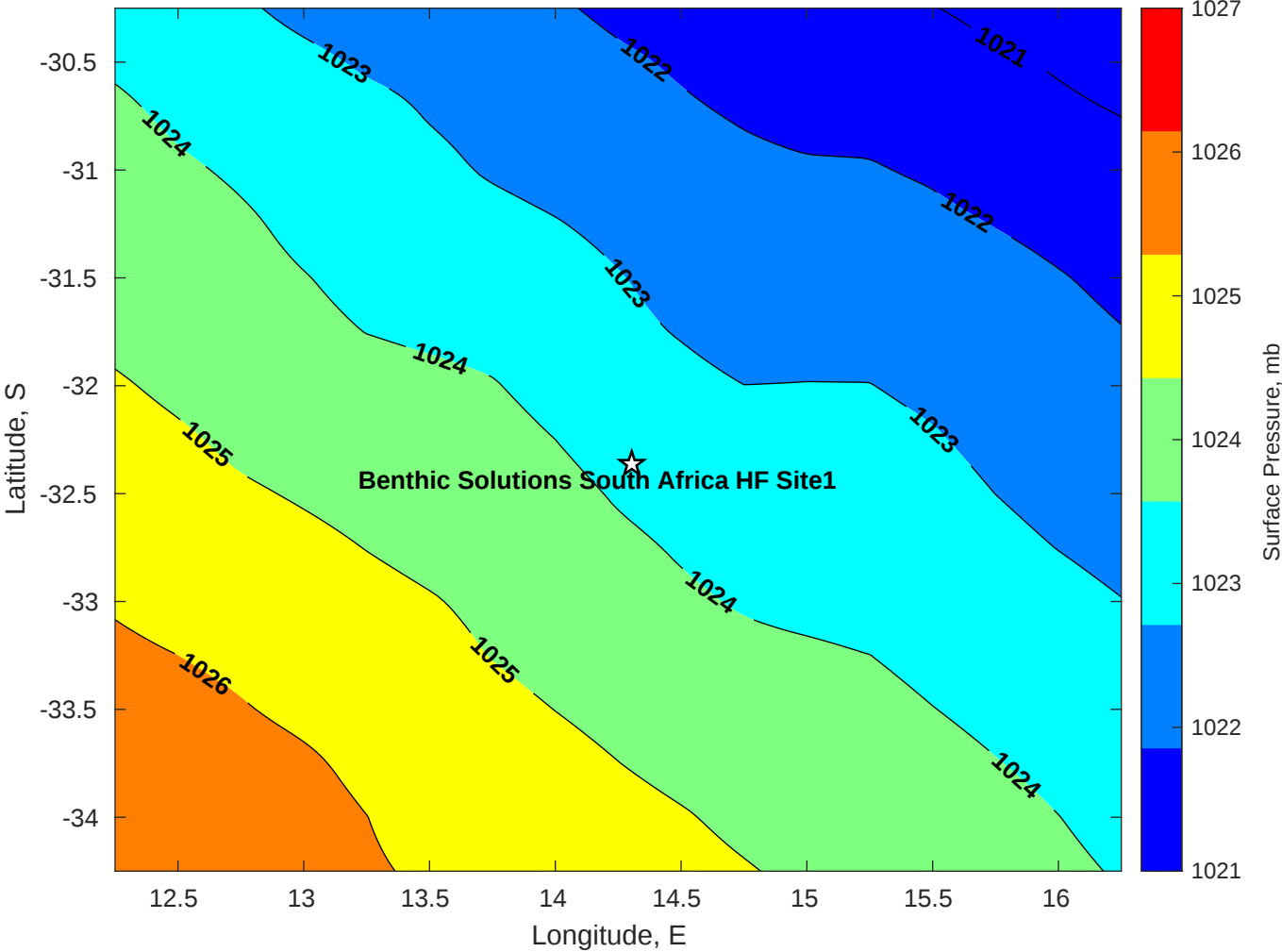
Surface Pressure (mb) for Benthic Solutions South Africa HF Site1 at 15-Apr-2025 00:00:00
