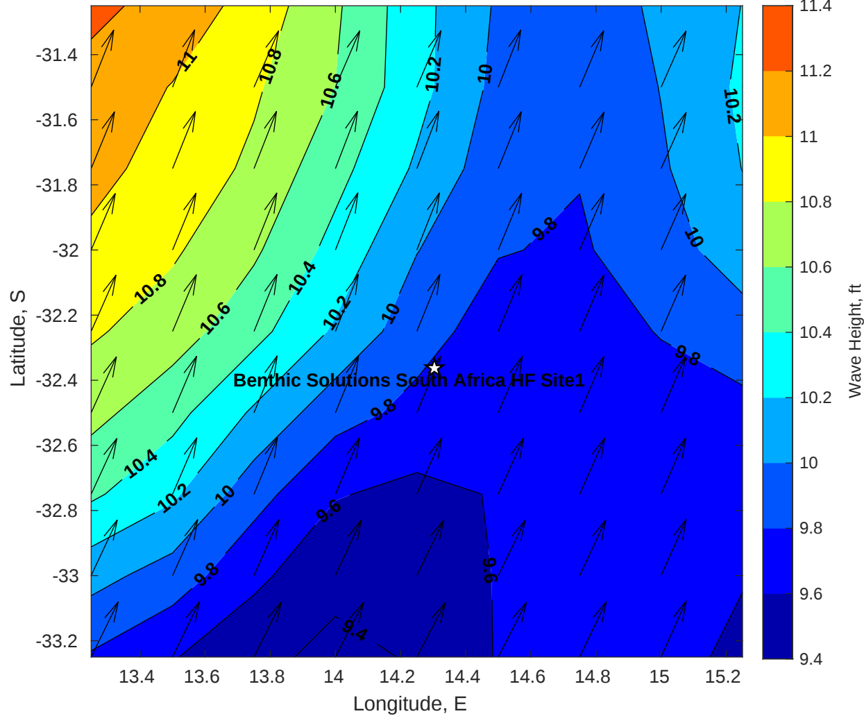
Wave Height (ft) for Benthic Solutions South Africa HF Site1 at 15-Apr-2025 09:00:00
