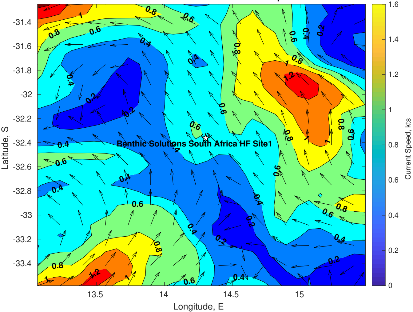
Surface Currents for Benthic Solutions South Africa HF Site1 at 14-Apr-2025 00:00:00
