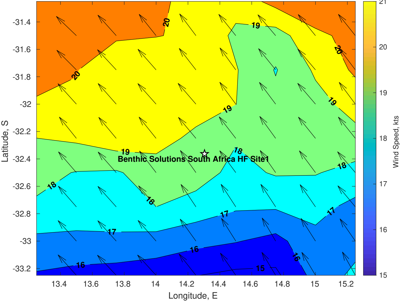
Winds (kts) for Benthic Solutions South Africa HF Site1 at 15-Apr-2025 09:00:00
