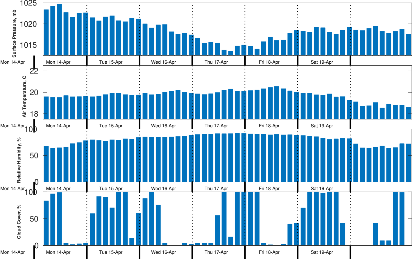
Met Forecast for Benthic Solutions South Africa HF Site1 from 15-Apr-2025 00:00:00 to 22-Apr-2025 00:00:00
