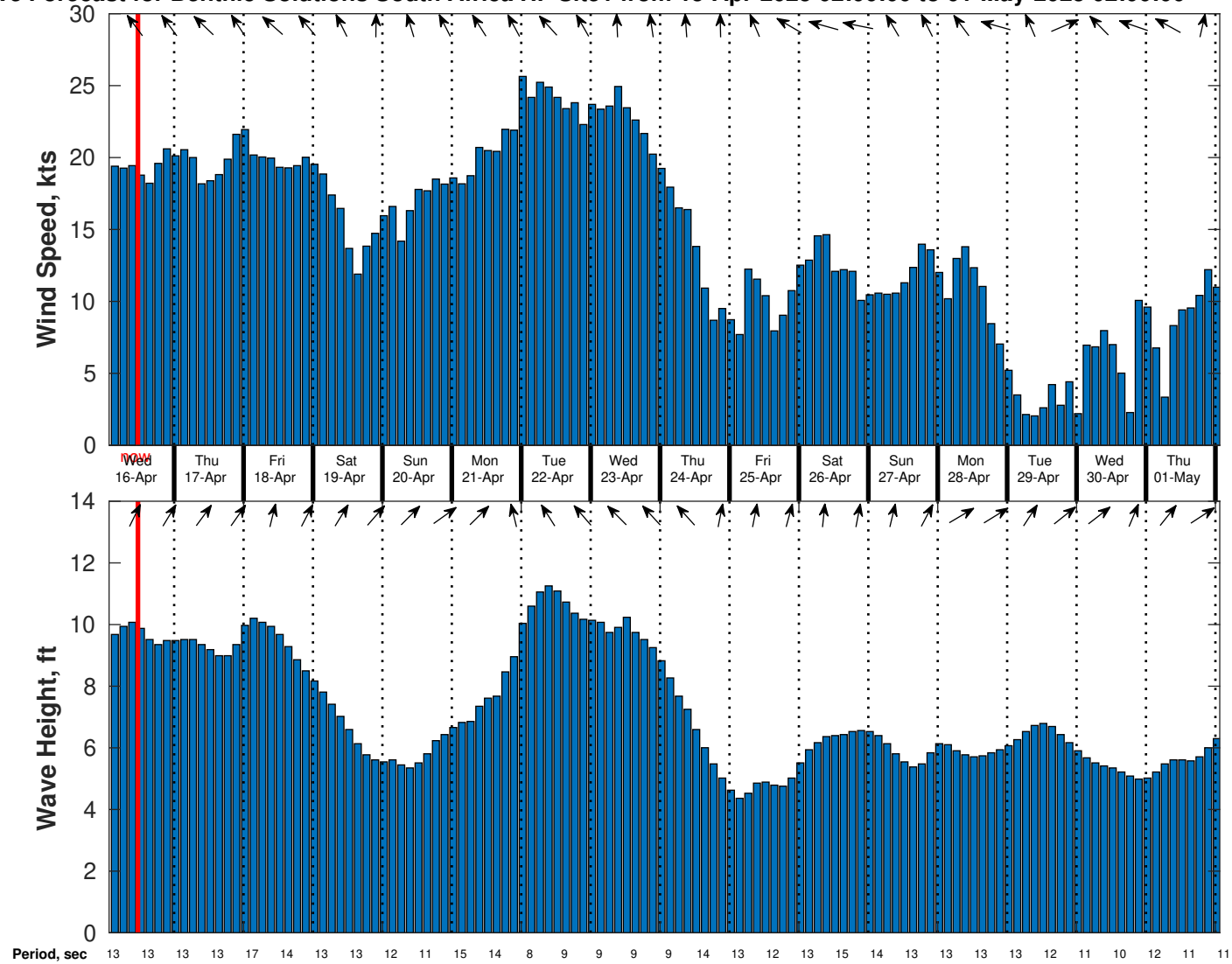
Wind & Wave Forecast for Benthic Solutions South Africa HF Site1 from 15-Apr-2025 02:00:00 to 01-May-2025 02:00:00
