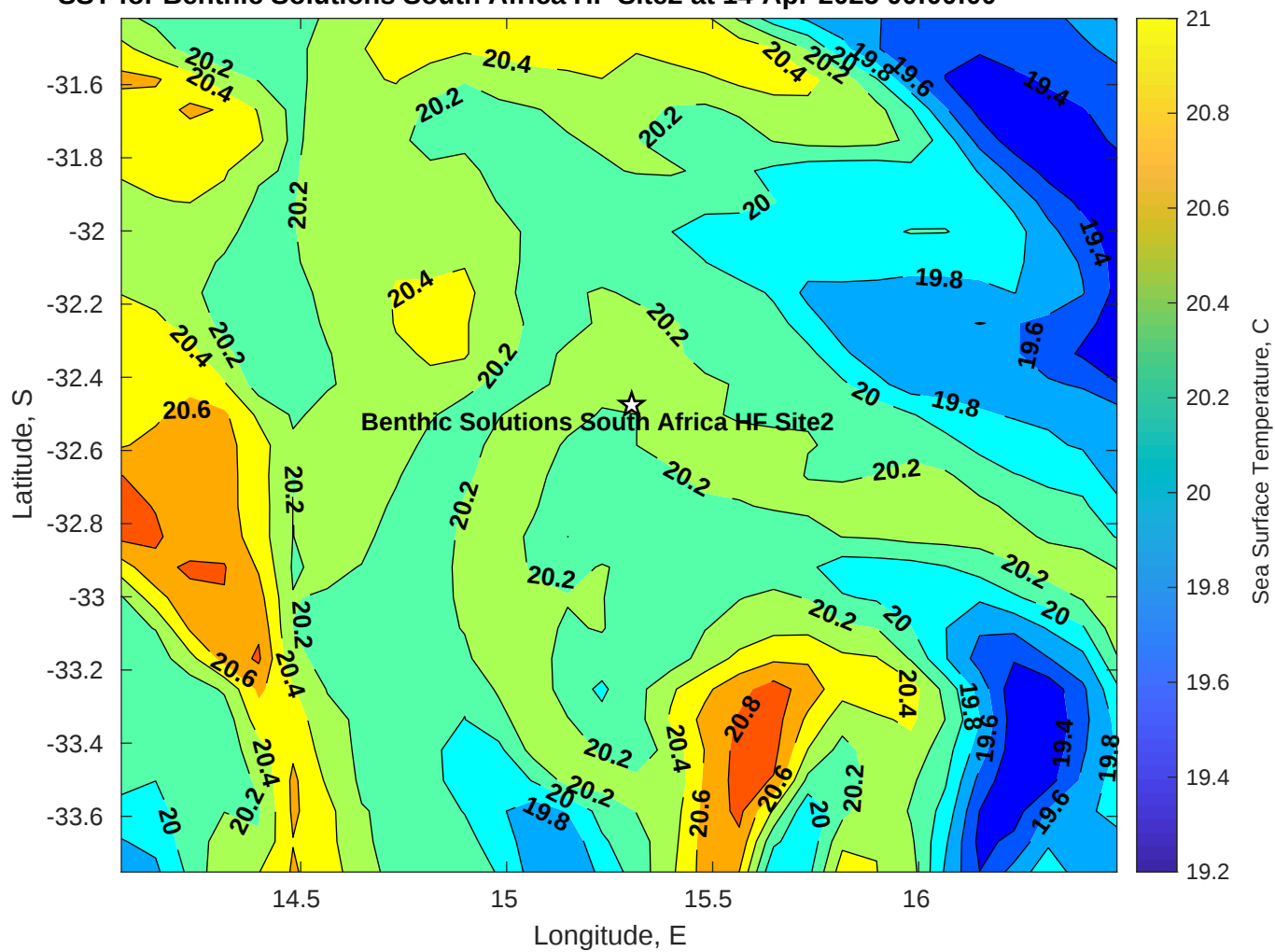
SST for Benthic Solutions South Africa HF Site2 at 14-Apr-2025 00:00:00
