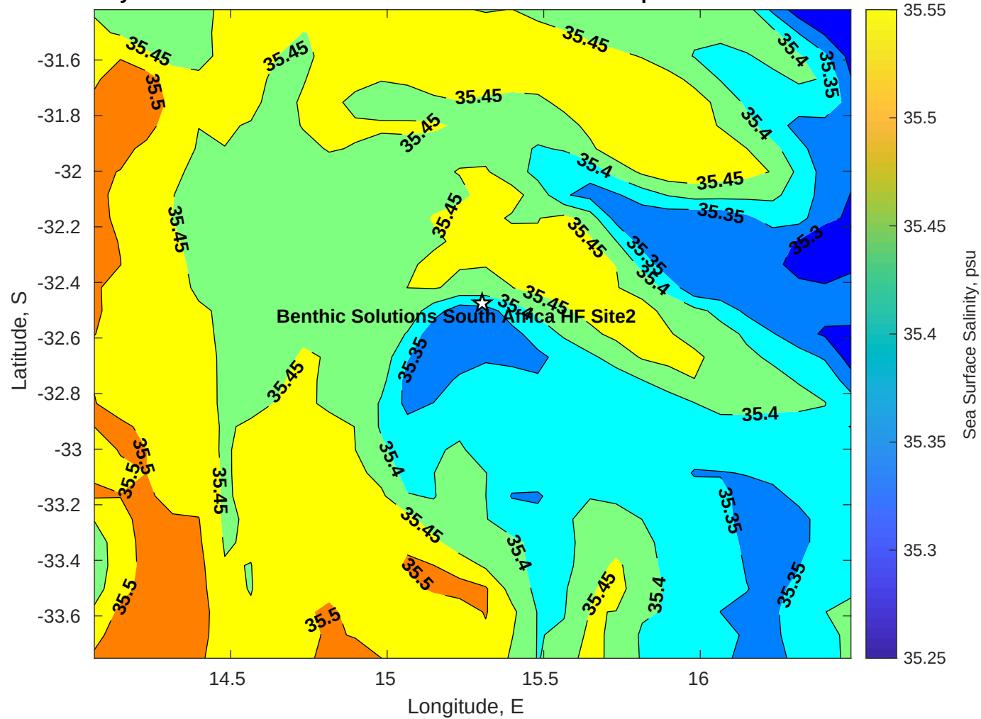
Surface Salinity for Benthic Solutions South Africa HF Site2 at 14-Apr-2025 00:00:00
